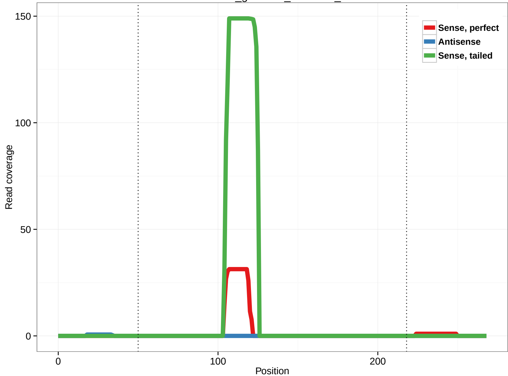
rheMac3_genscan_chr4.850_11
