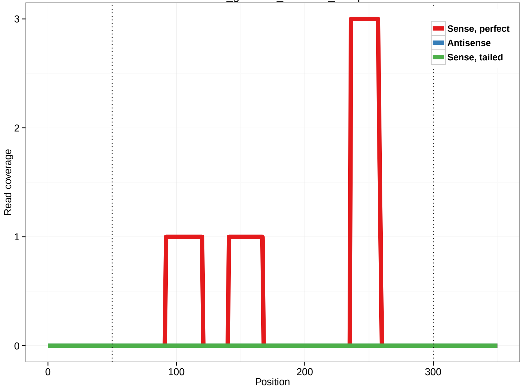
rheMac3_genscan_chr4.849_11.3p
