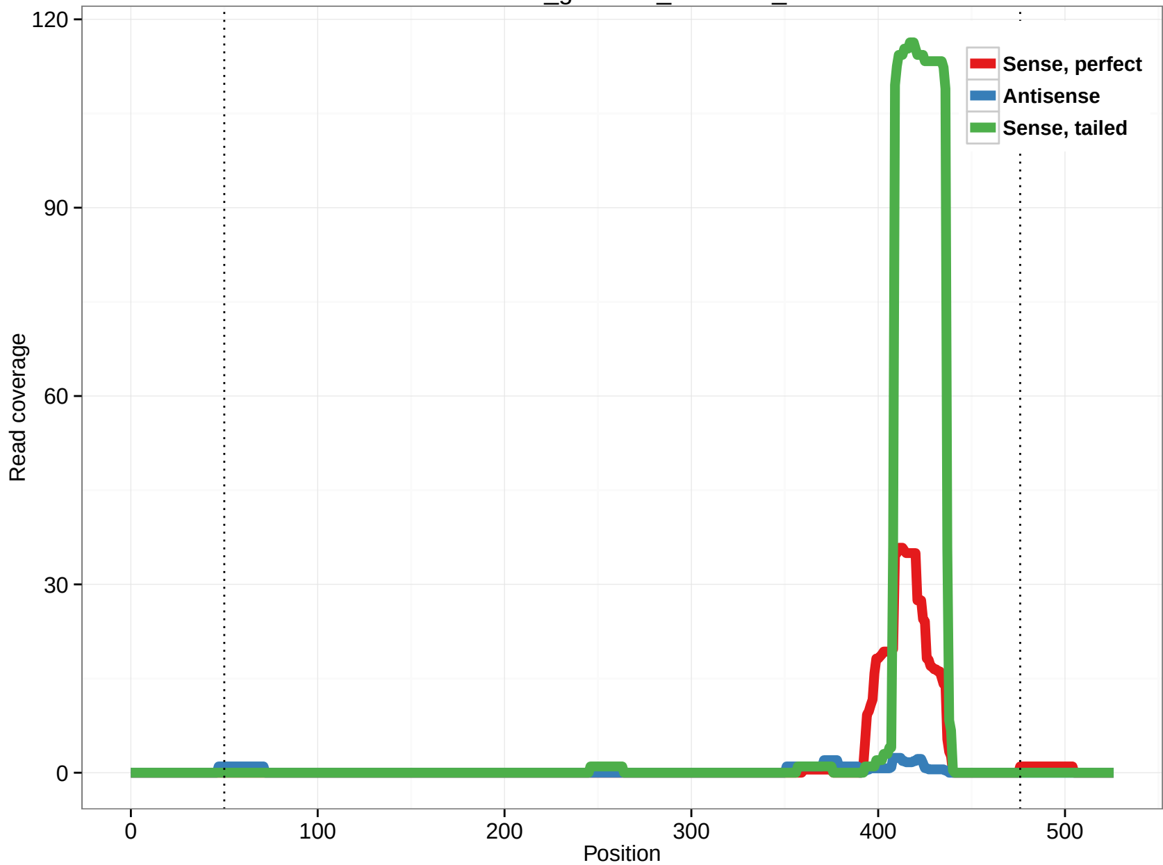
rheMac3_genscan_chr4.820_2
