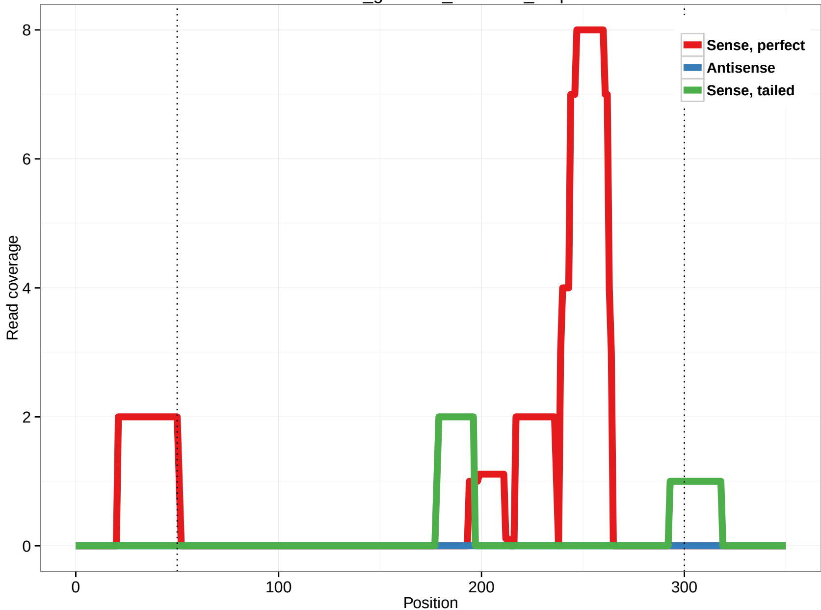
rheMac3_genscan_chr4.813_6.5p
