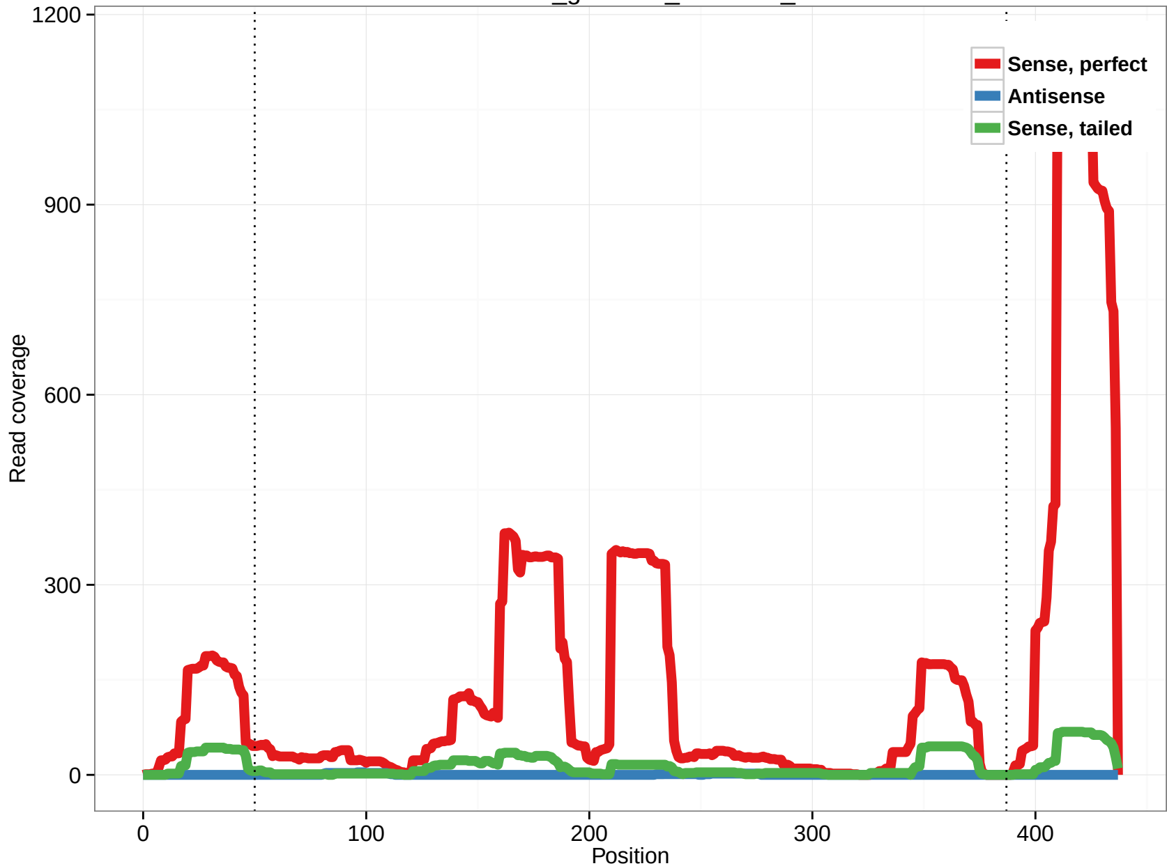
rheMac3_genscan_chr4.800_6
