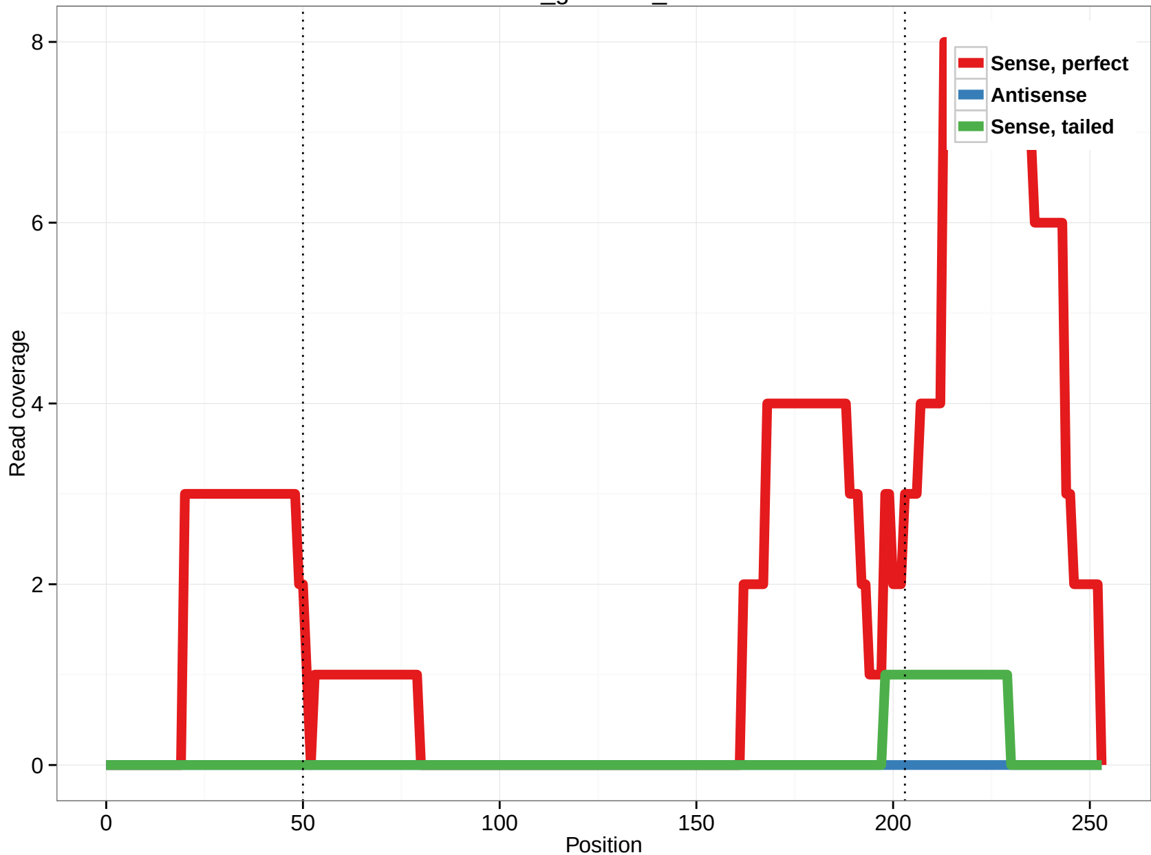
rheMac3_genscan_chr4.740
