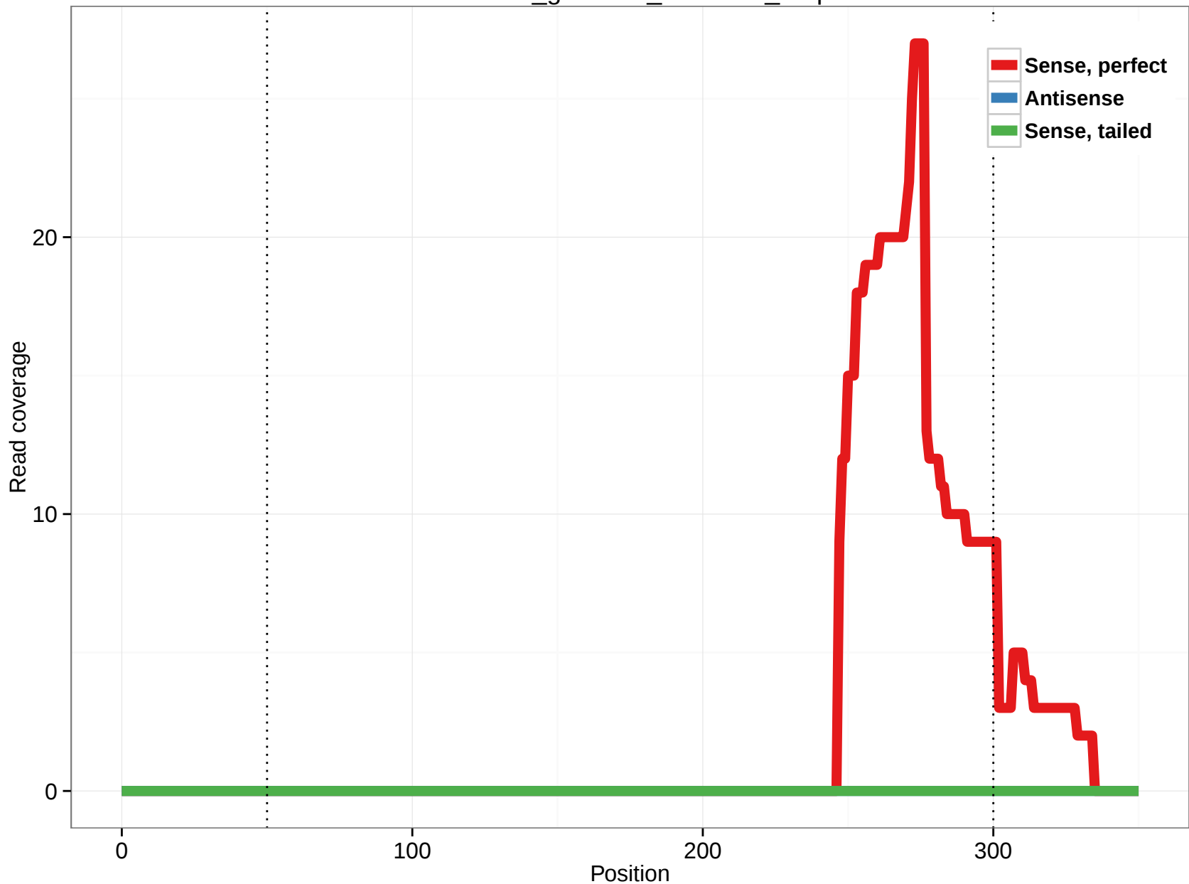
rheMac3_genscan_chr4.733_2.3p
