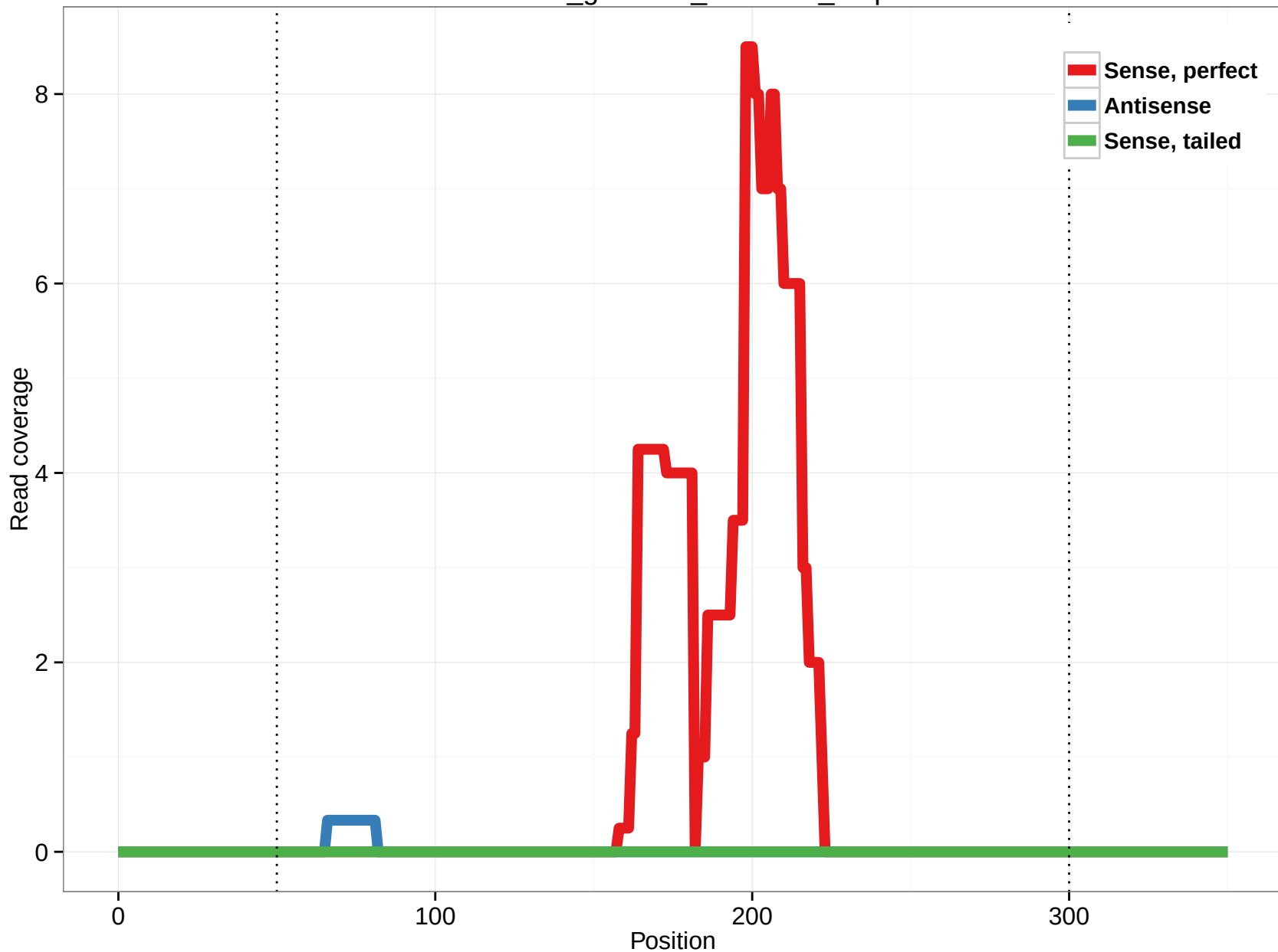
rheMac3_genscan_chr4.731_1.3p
