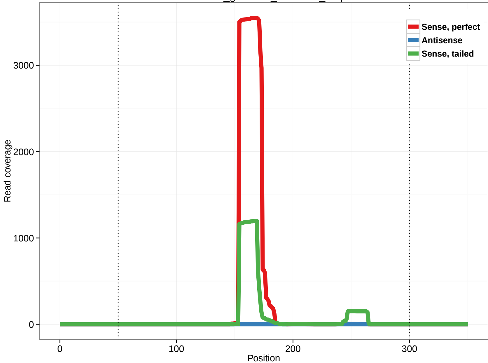
rheMac3_genscan_chr4.716_7.3p
