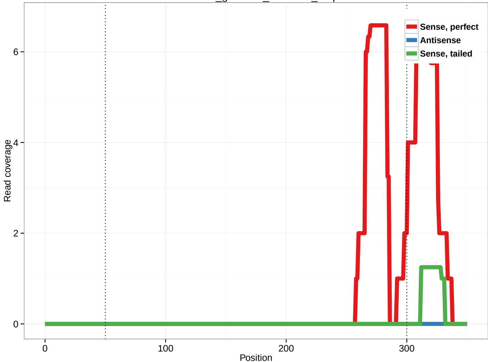
rheMac3_genscan_chr4.641_3.3p
