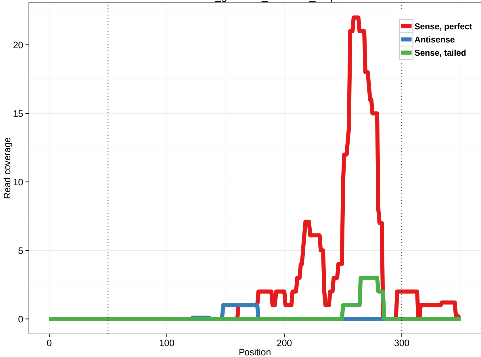
rheMac3_genscan_chr4.641_1.3p
