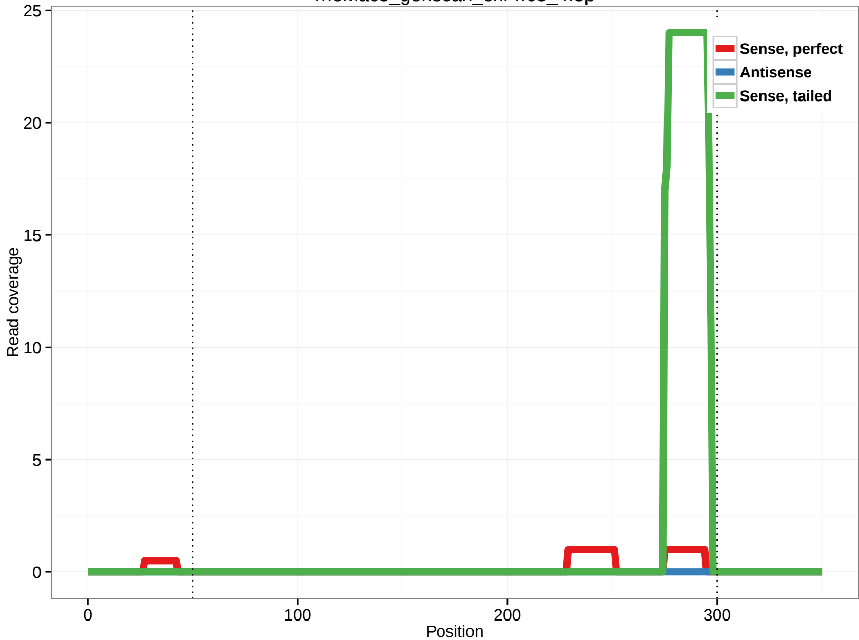
rheMac3_genscan_chr4.63_4.3p
