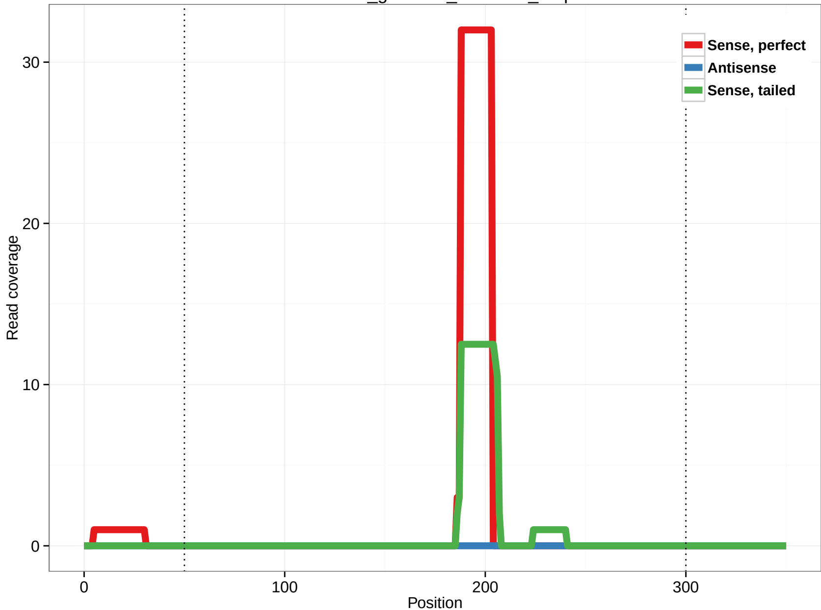
rheMac3_genscan_chr4.566_2.5p
