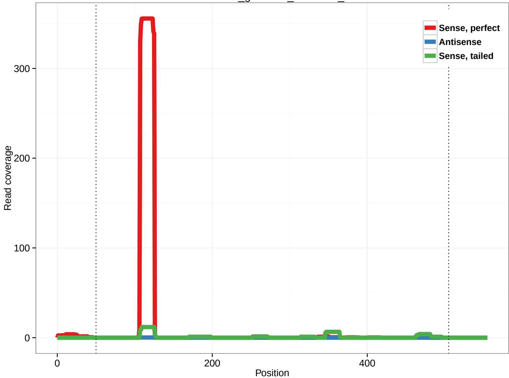
rheMac3_genscan_chr4.488_5
