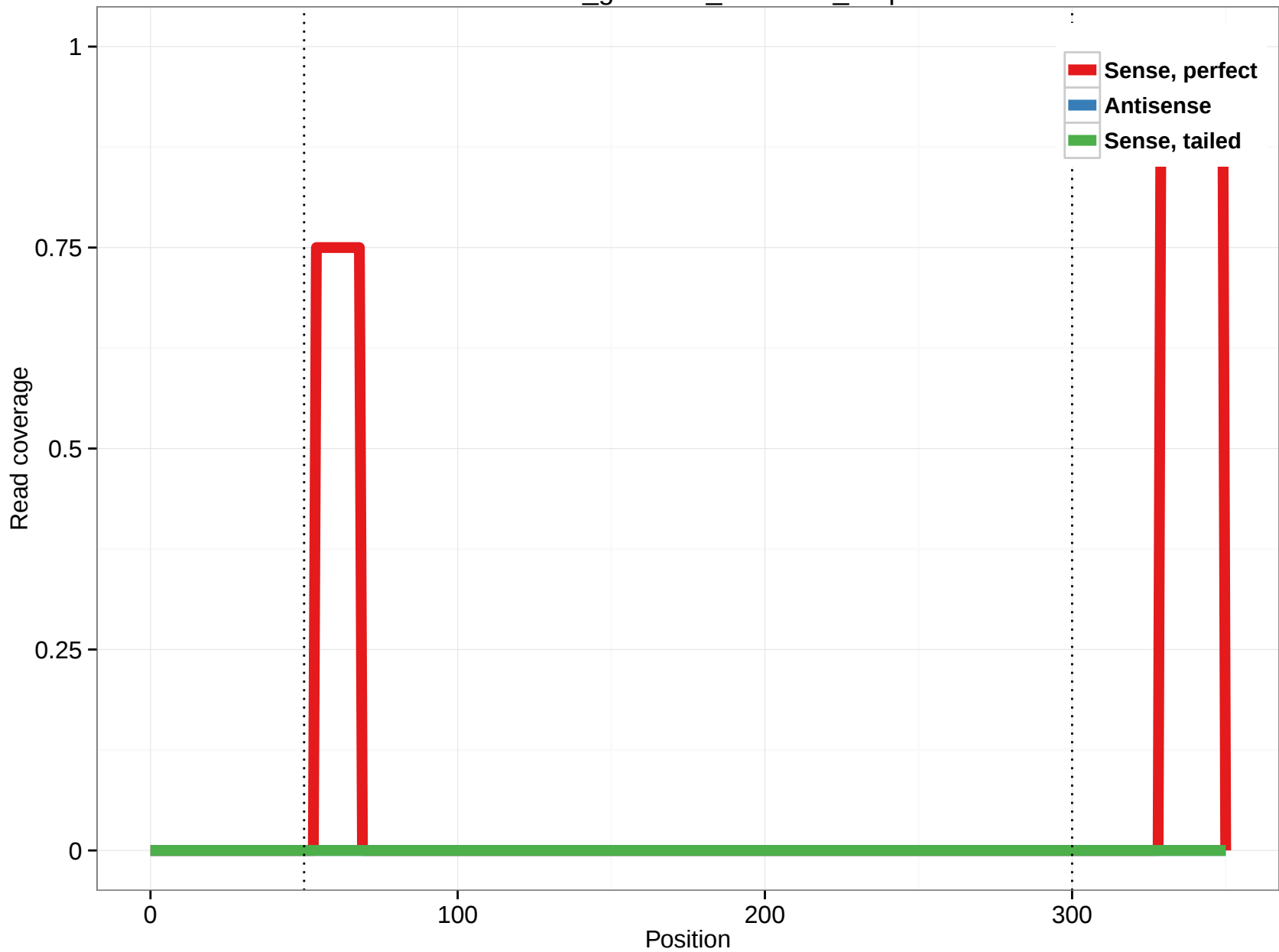
rheMac3_genscan_chr4.465_3.3p
