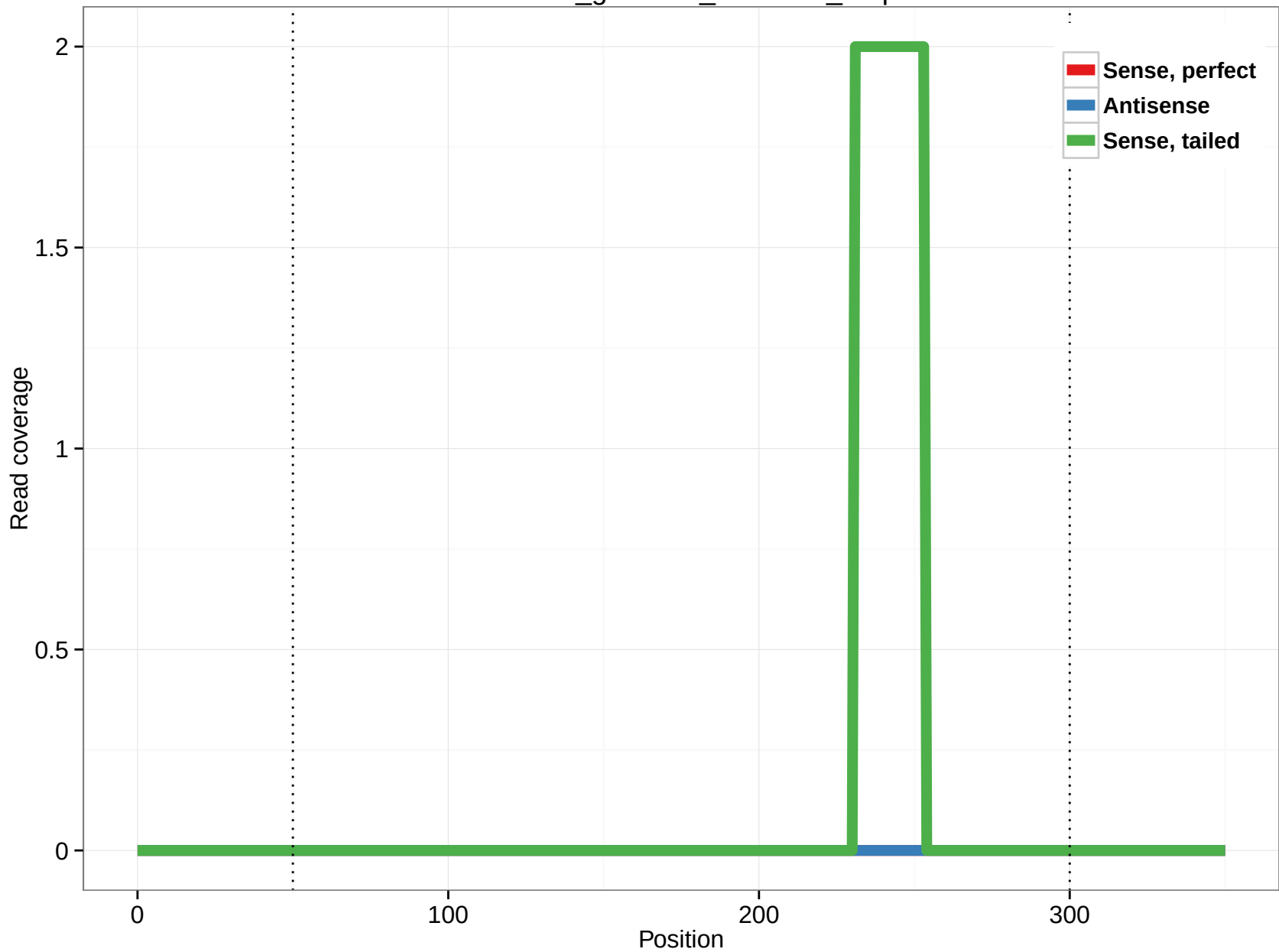
rheMac3_genscan_chr4.421_4.3p
