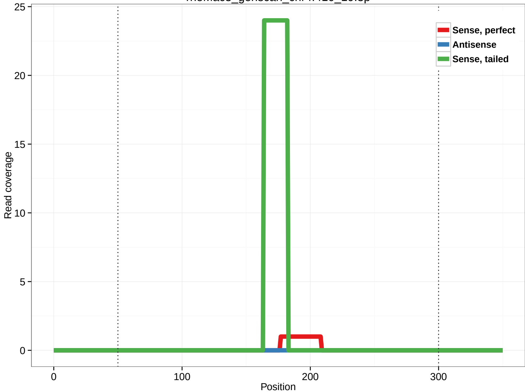
rheMac3_genscan_chr4.410_19.3p
