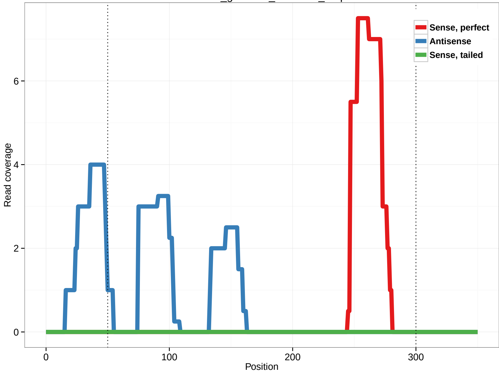
rheMac3_genscan_chr4.349_1.5p
