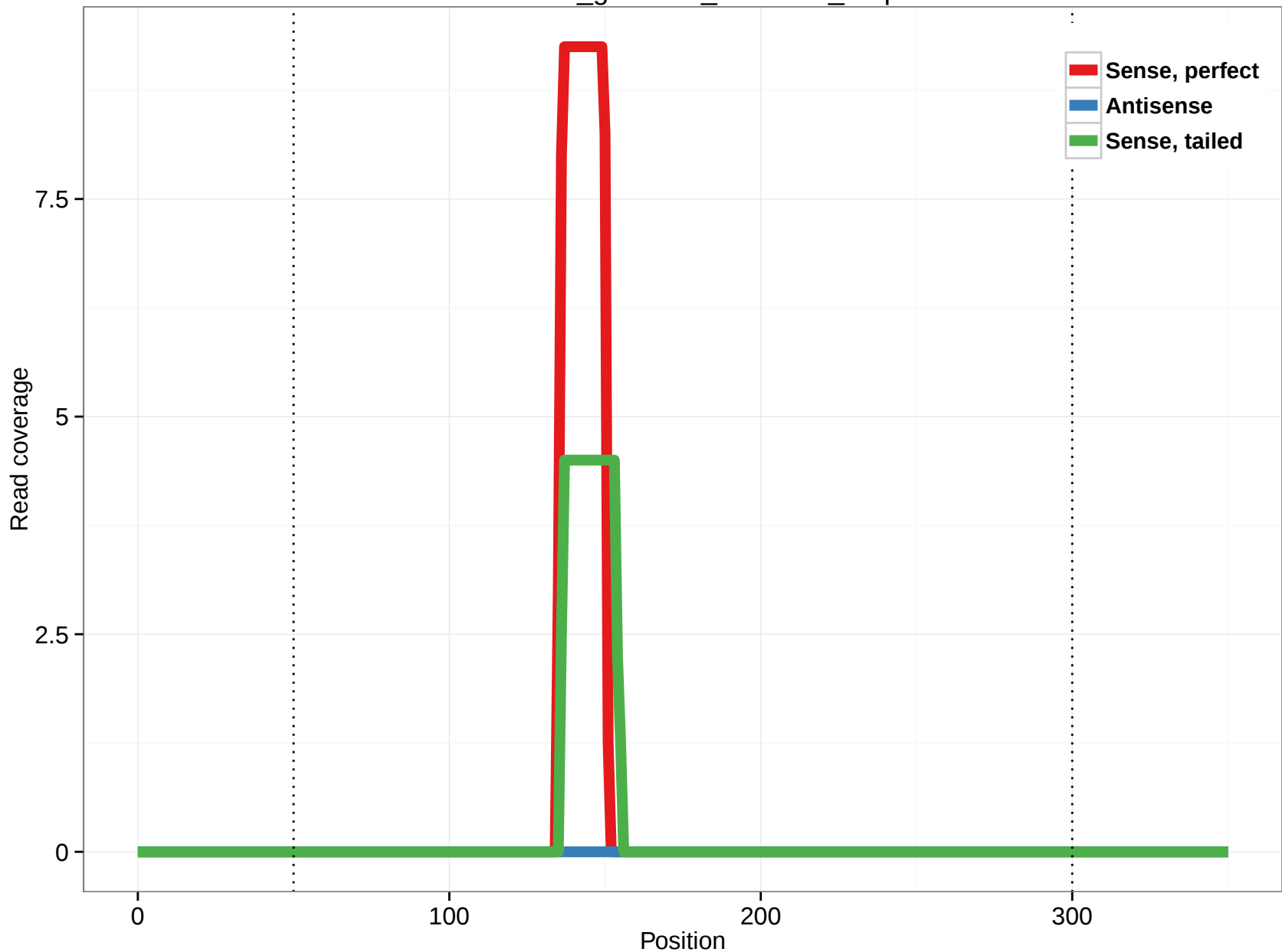
rheMac3_genscan_chr4.346_0.5p
