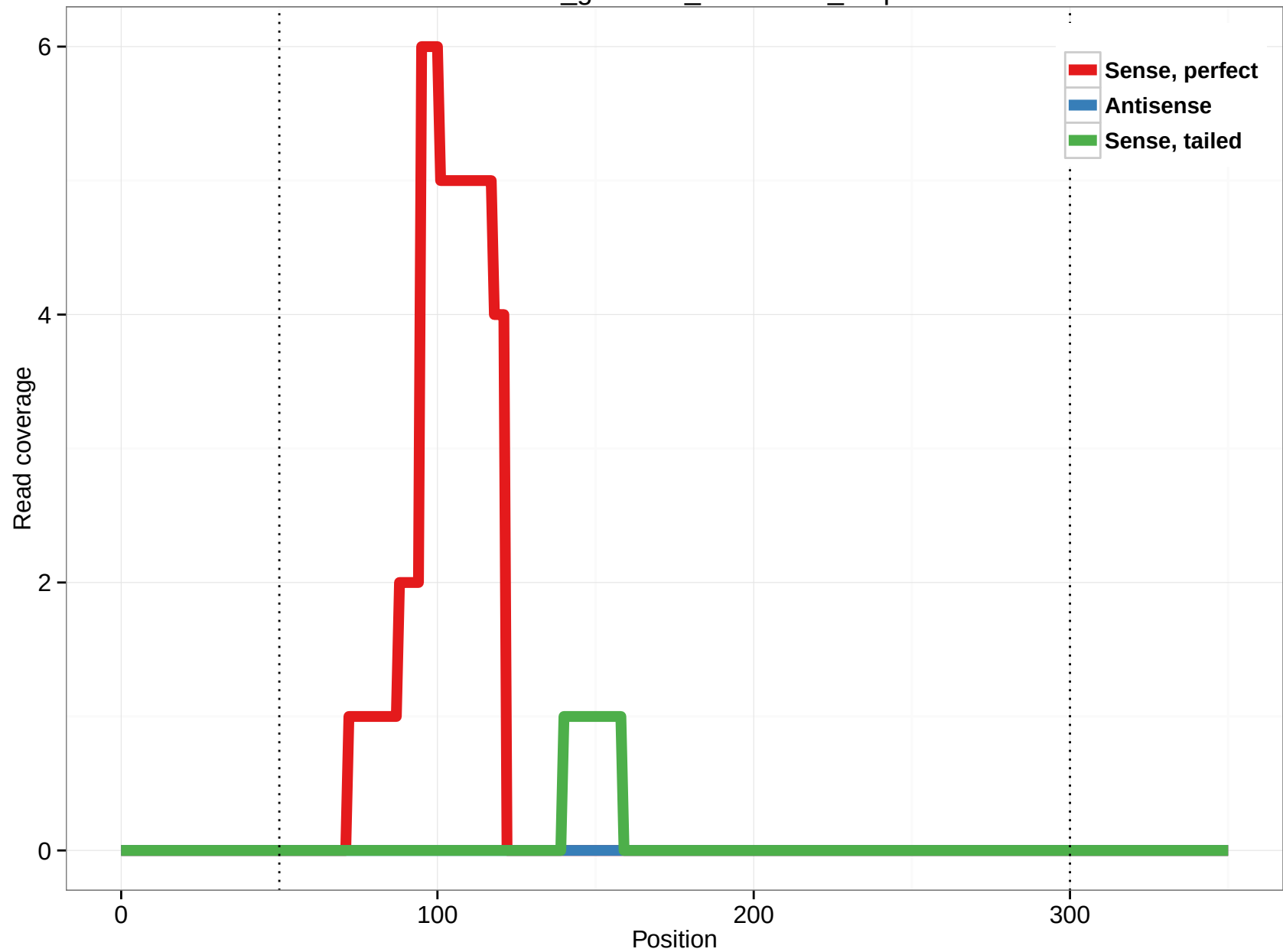
rheMac3_genscan_chr4.3445_2.3p
