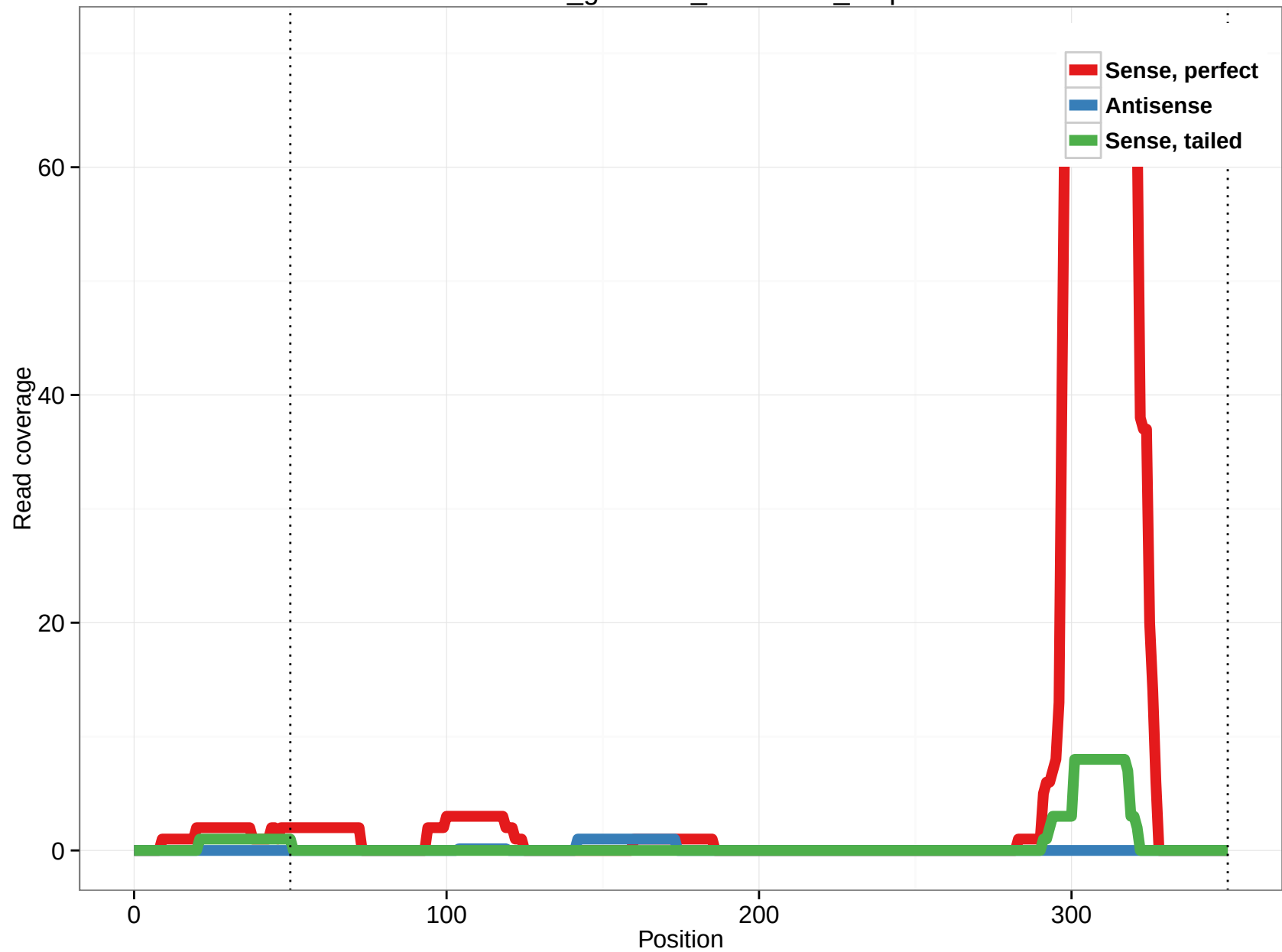
rheMac3_genscan_chr4.3445_1.5p
