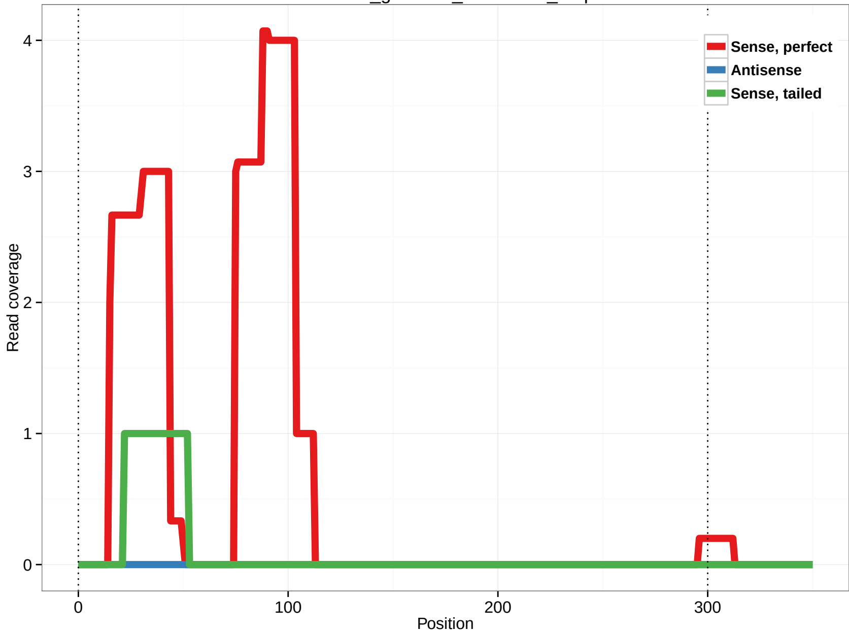
rheMac3_genscan_chr4.3443_2.3p
