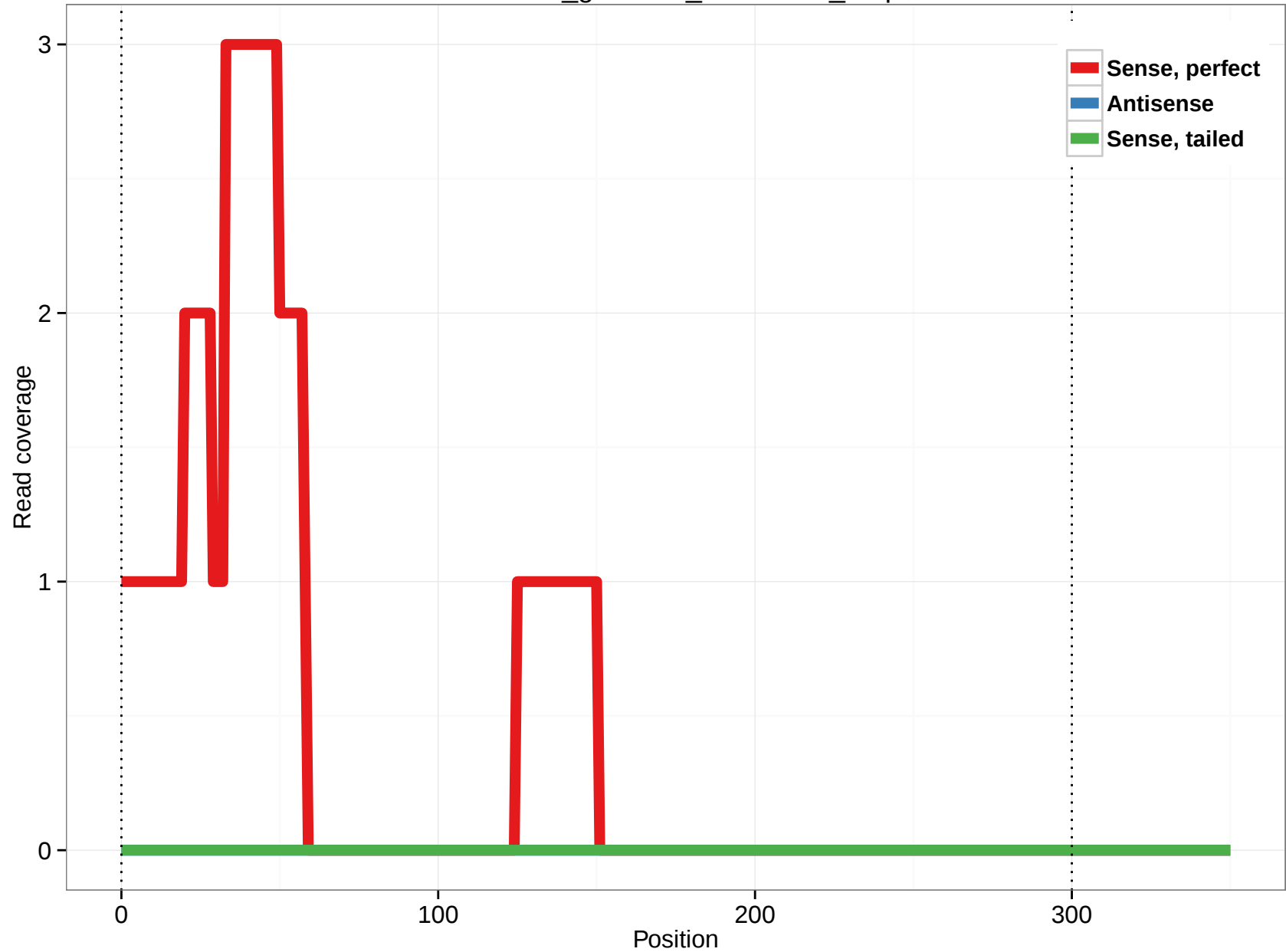
rheMac3_genscan_chr4.3442_0.3p
