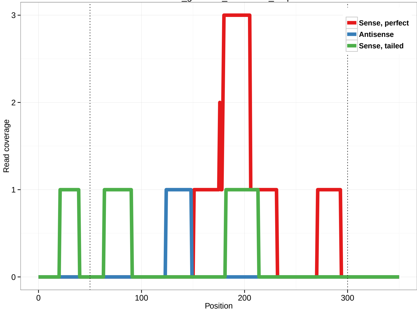
rheMac3_genscan_chr4.3390_3.5p
