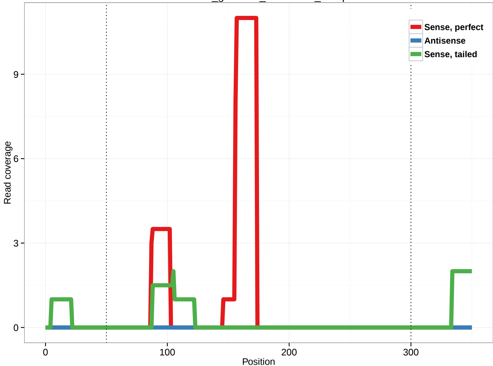
rheMac3_genscan_chr4.3379_36.5p
