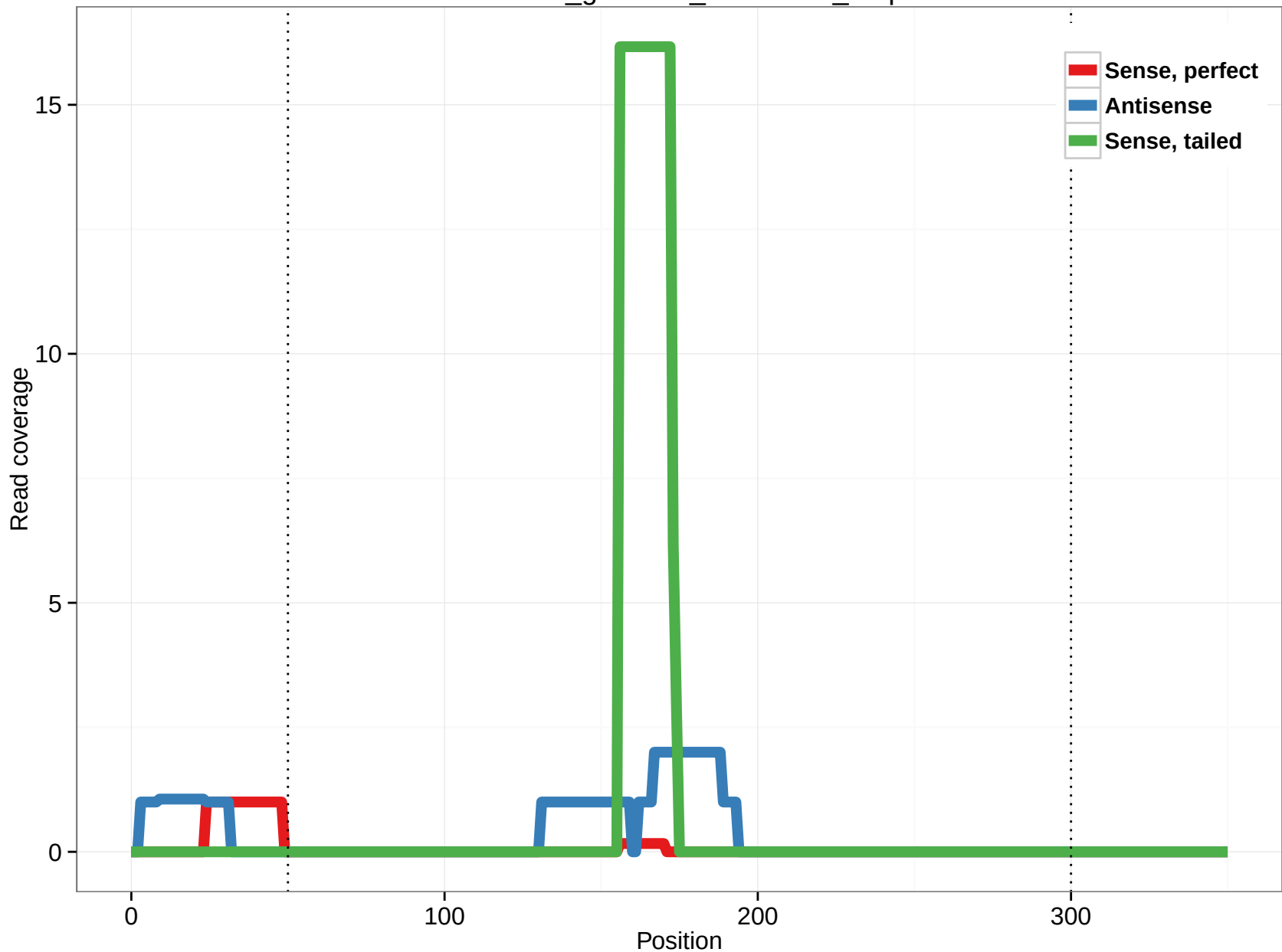
rheMac3_genscan_chr4.3158_0.5p
