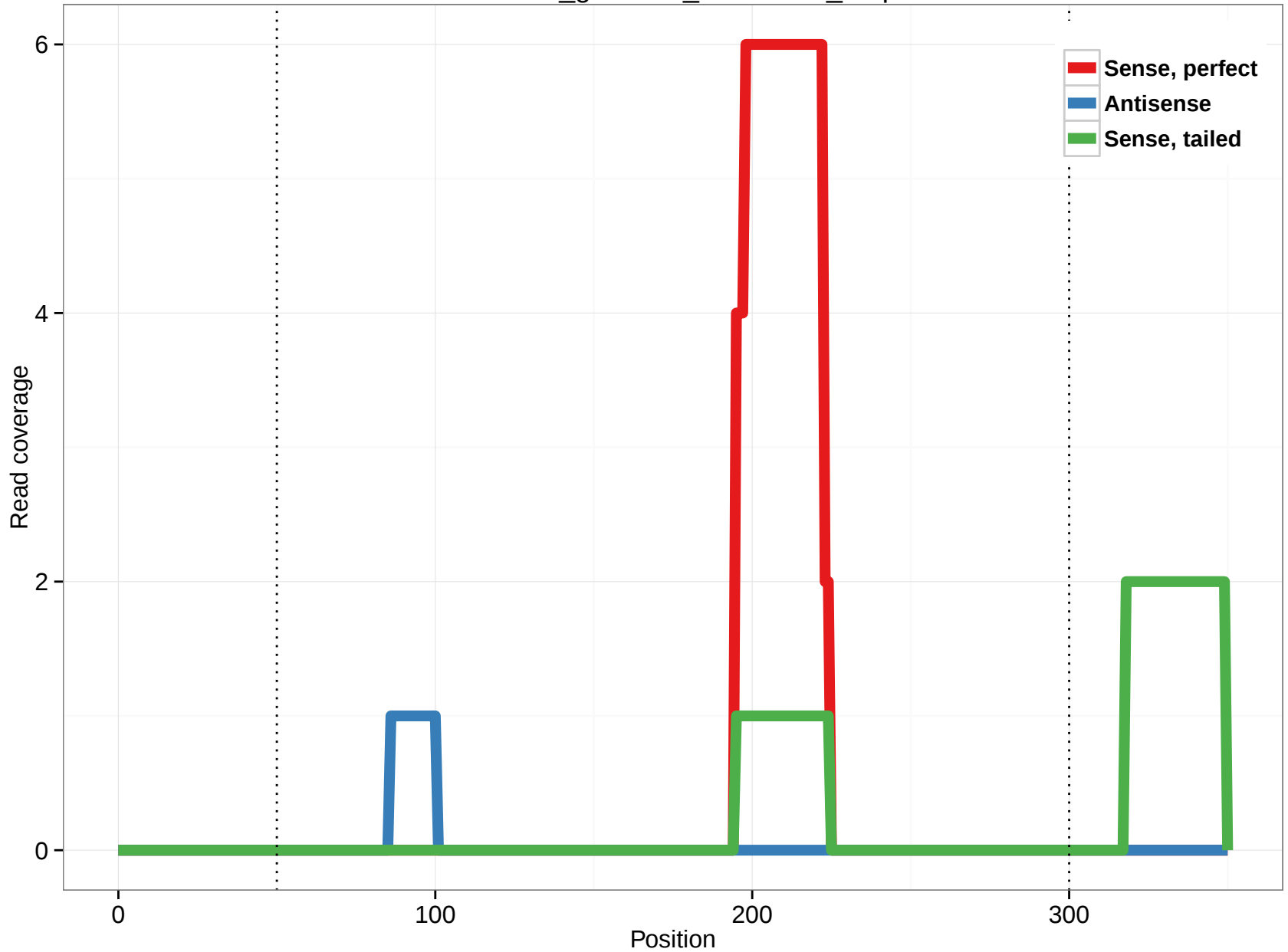
rheMac3_genscan_chr4.3060_1.5p
