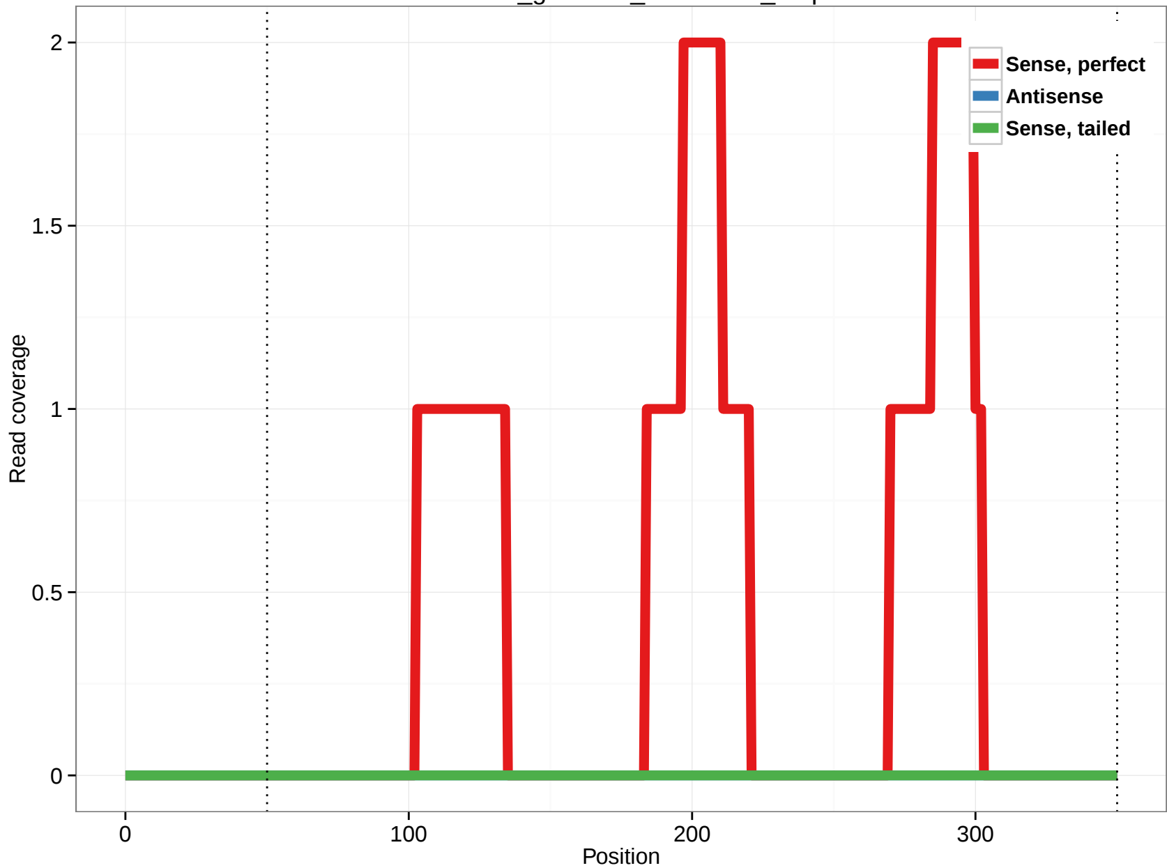
rheMac3_genscan_chr4.3058_6.5p
