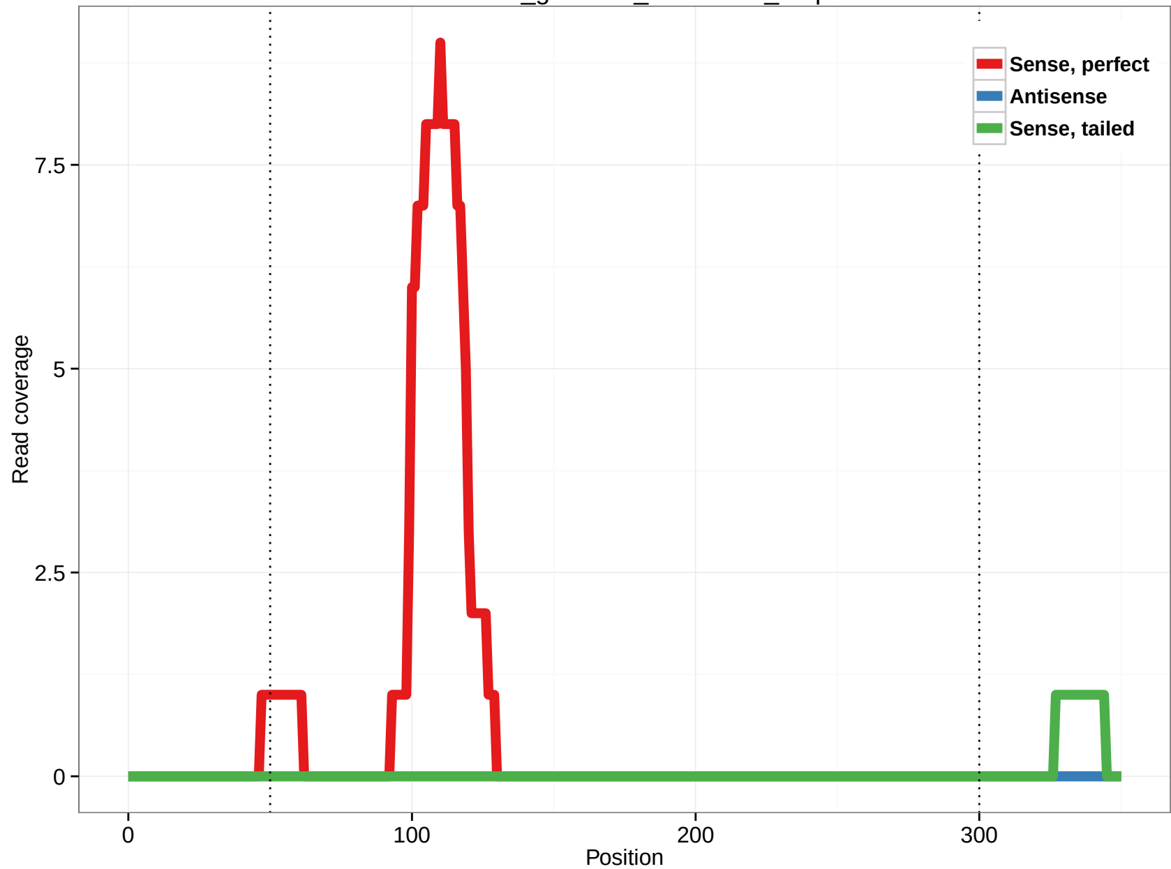
rheMac3_genscan_chr4.3041_6.5p
