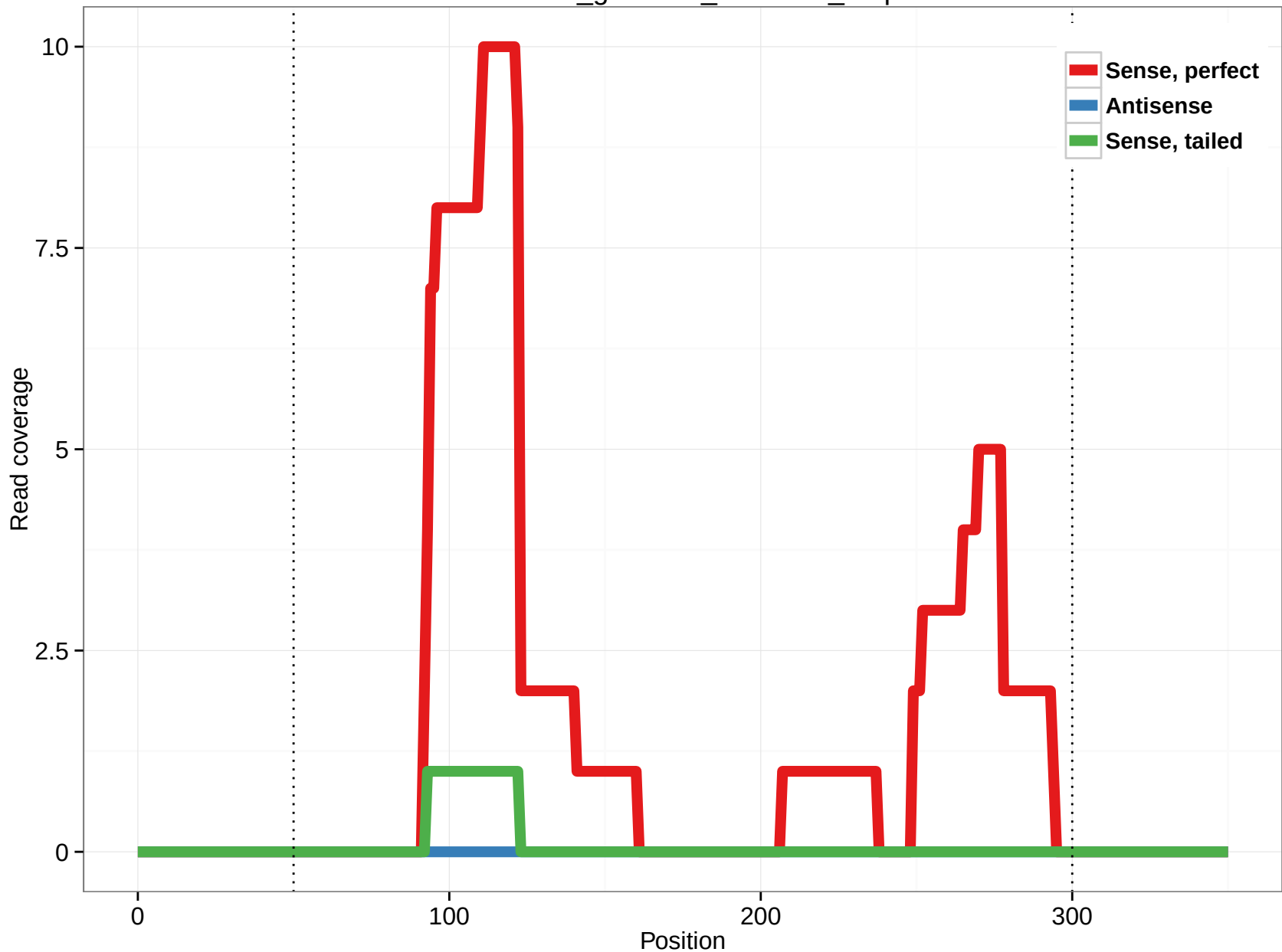
rheMac3_genscan_chr4.303_3.5p
