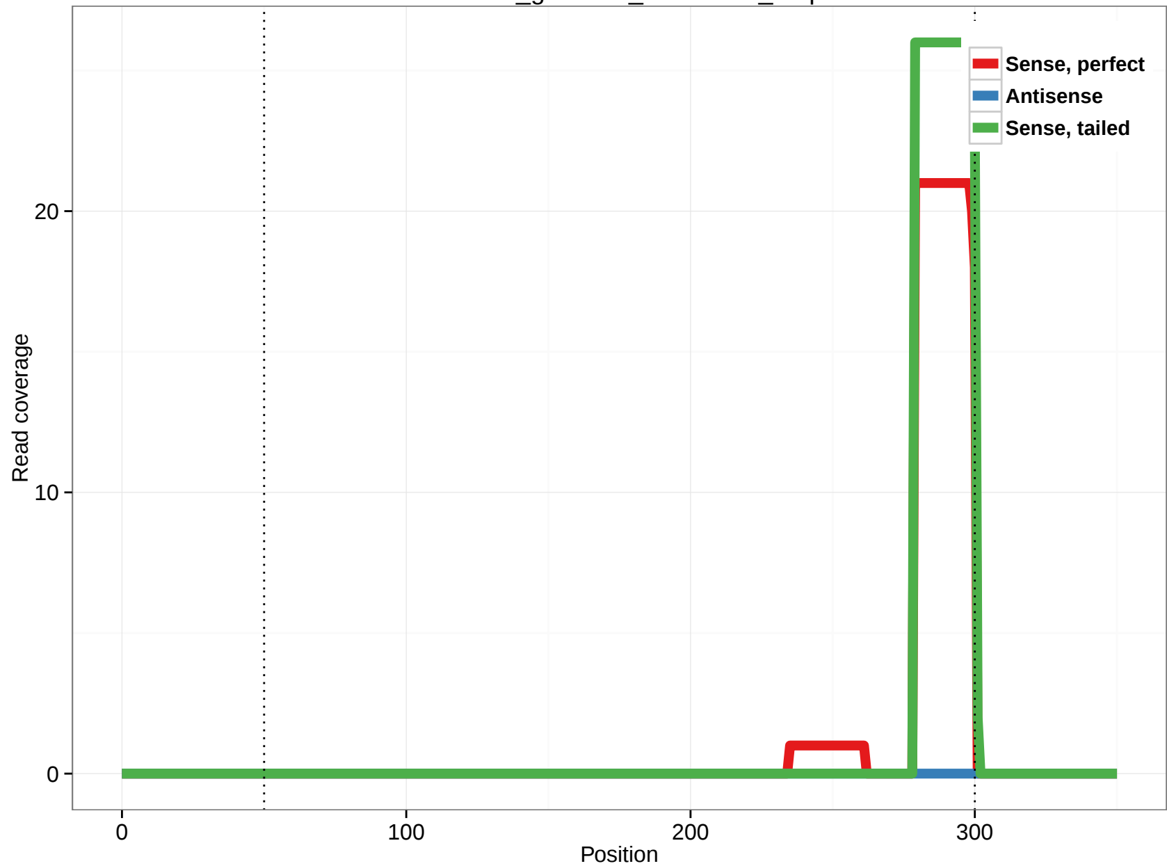
rheMac3_genscan_chr4.3025_9.3p
