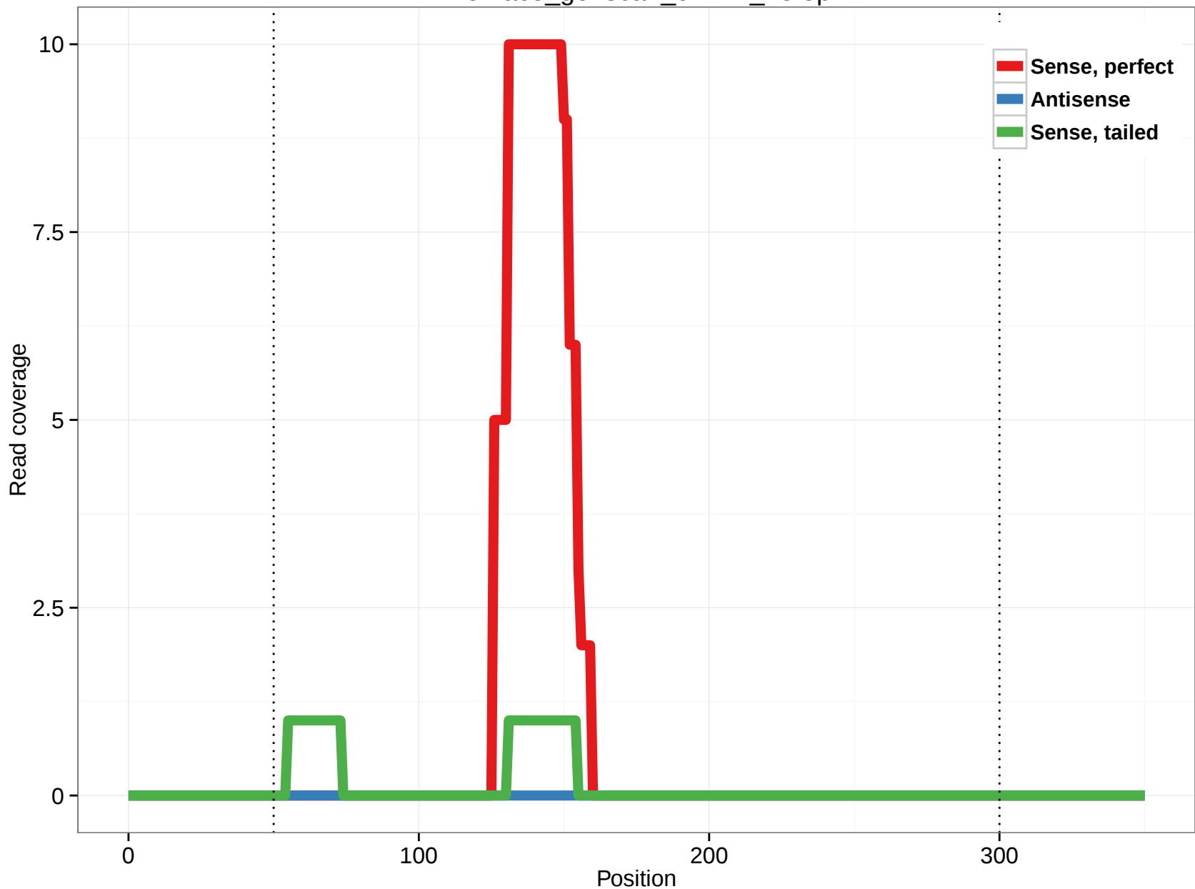
rheMac3_genscan_chr4.2_15.5p
