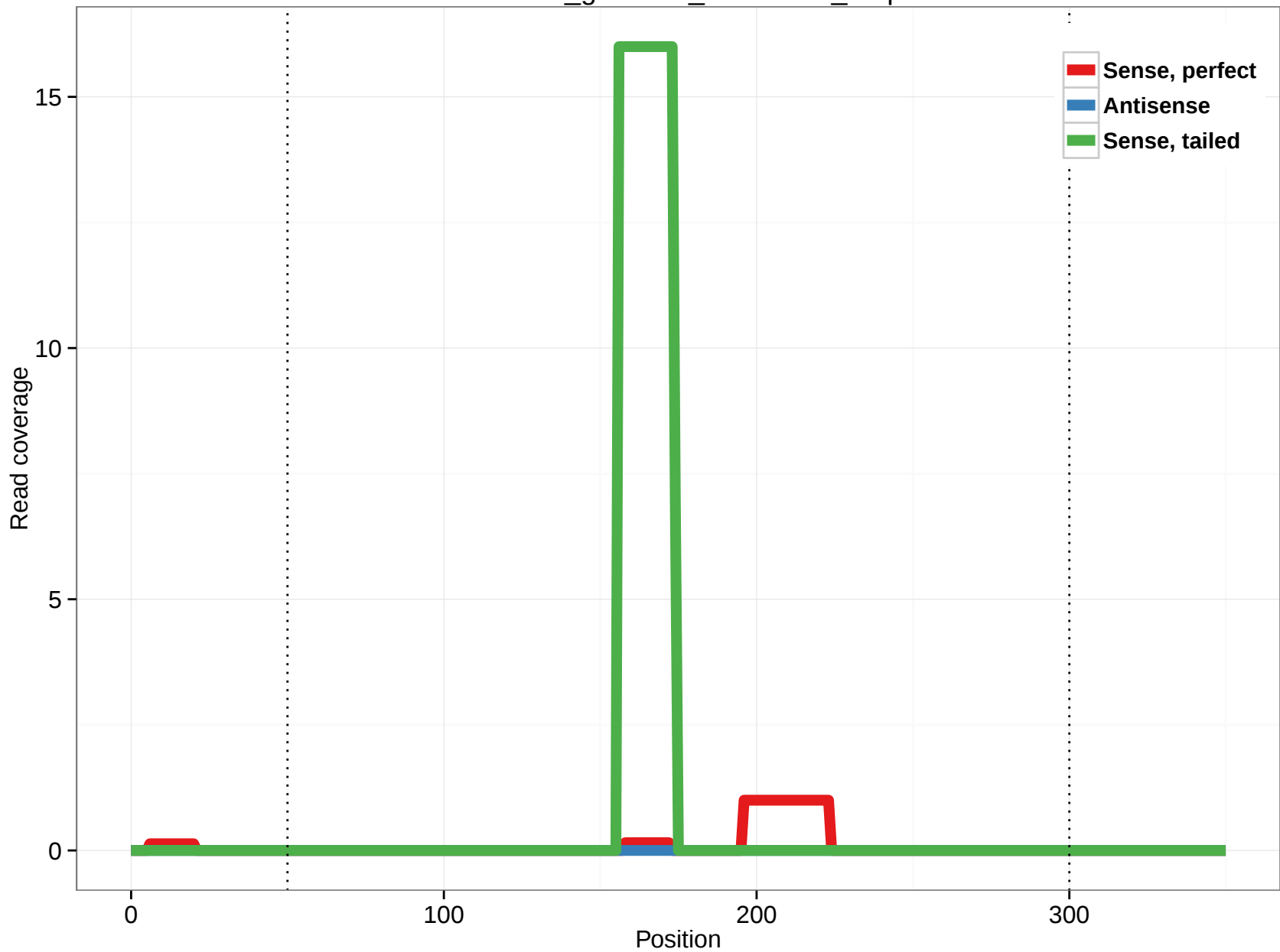
rheMac3_genscan_chr4.2895_5.3p
