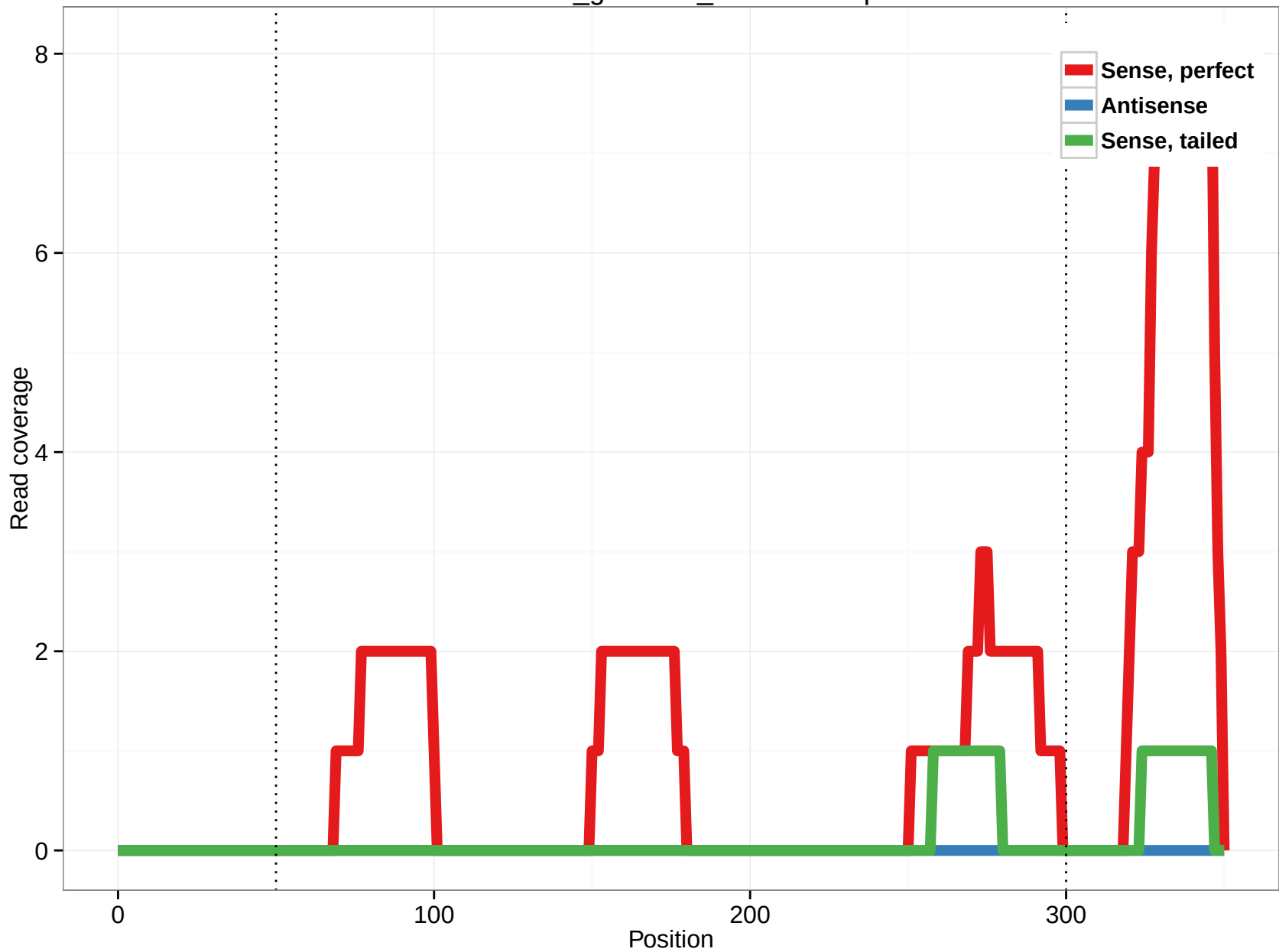
rheMac3_genscan_chr4.2873.5p
