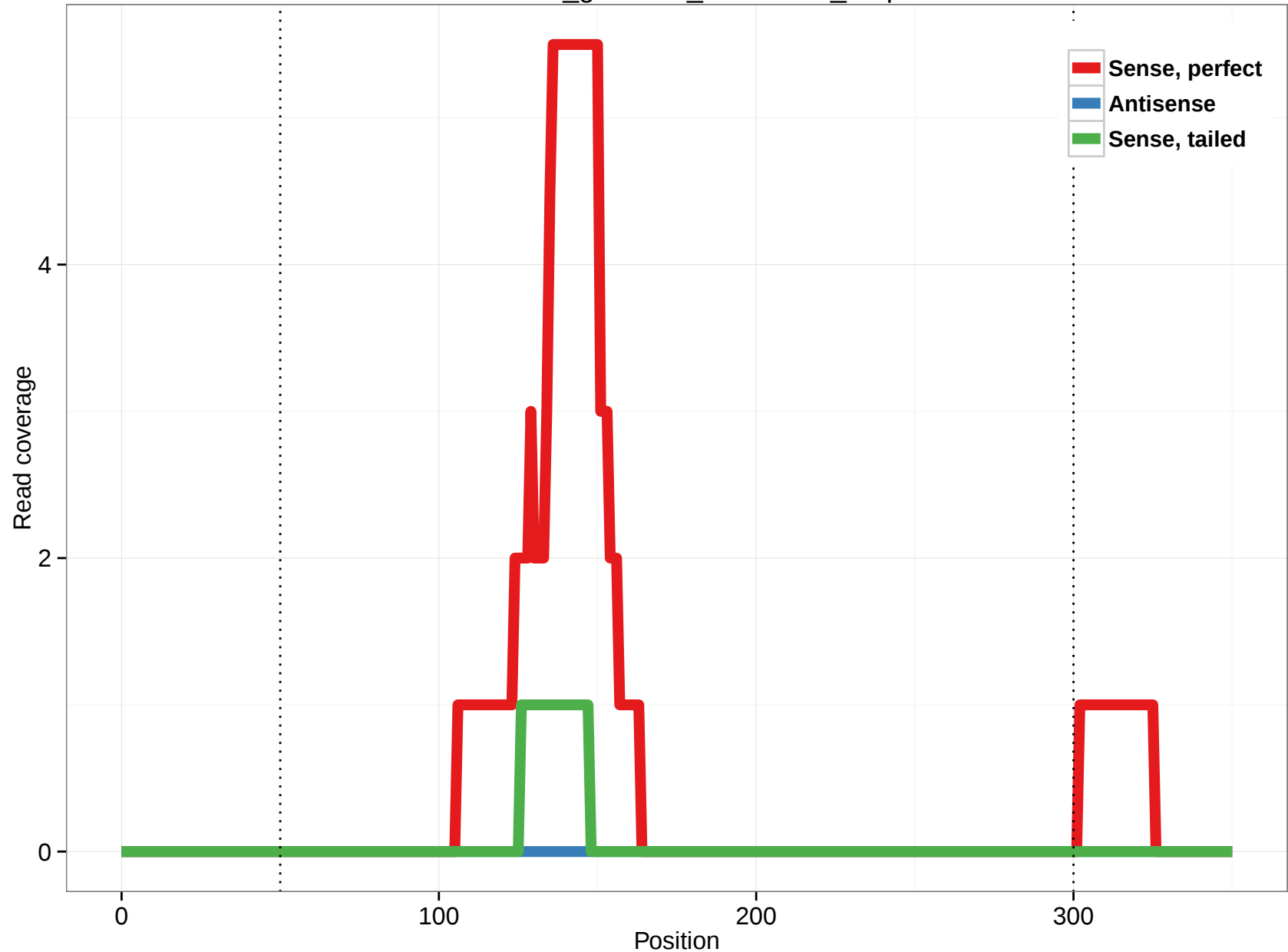
rheMac3_genscan_chr4.2854_3.3p
