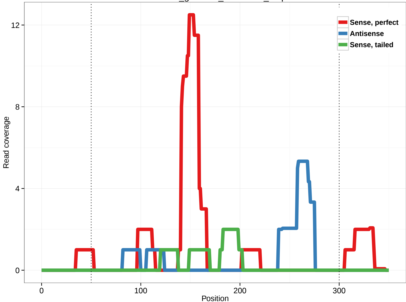
rheMac3_genscan_chr4.2850_4.5p
