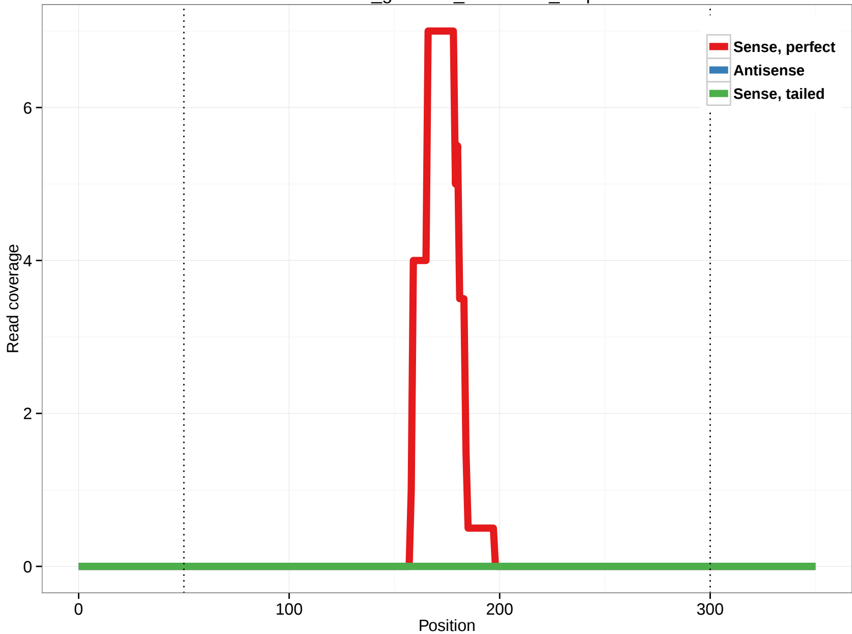
rheMac3_genscan_chr4.2787_0.3p
