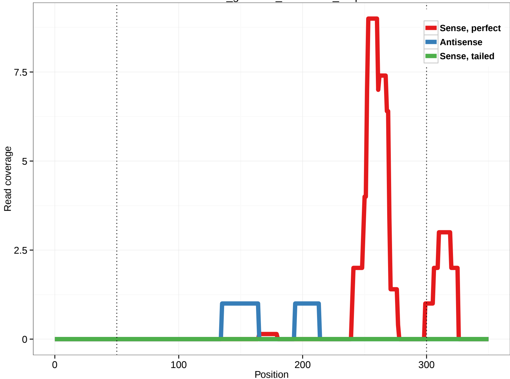
rheMac3_genscan_chr4.2631_0.3p
