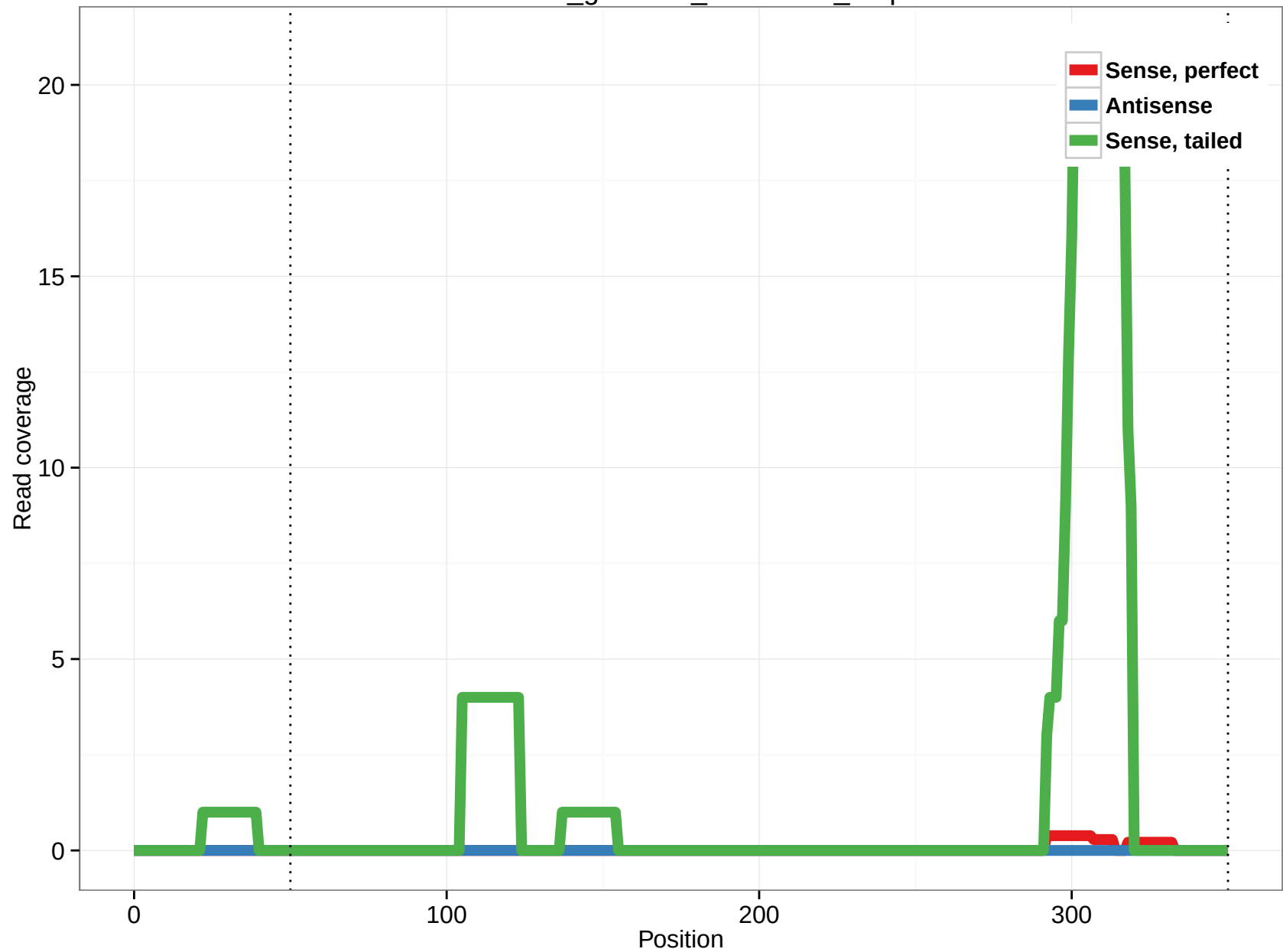
rheMac3_genscan_chr4.2597_0.5p
