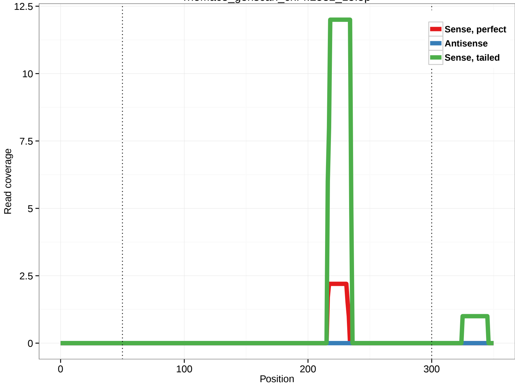
rheMac3_genscan_chr4.2532_15.5p
