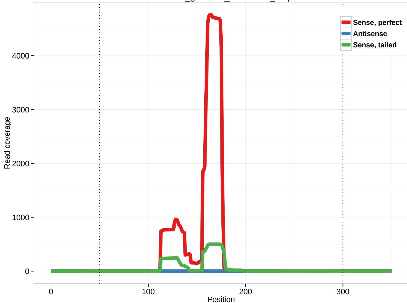
rheMac3_genscan_chr4.2489_4.5p
