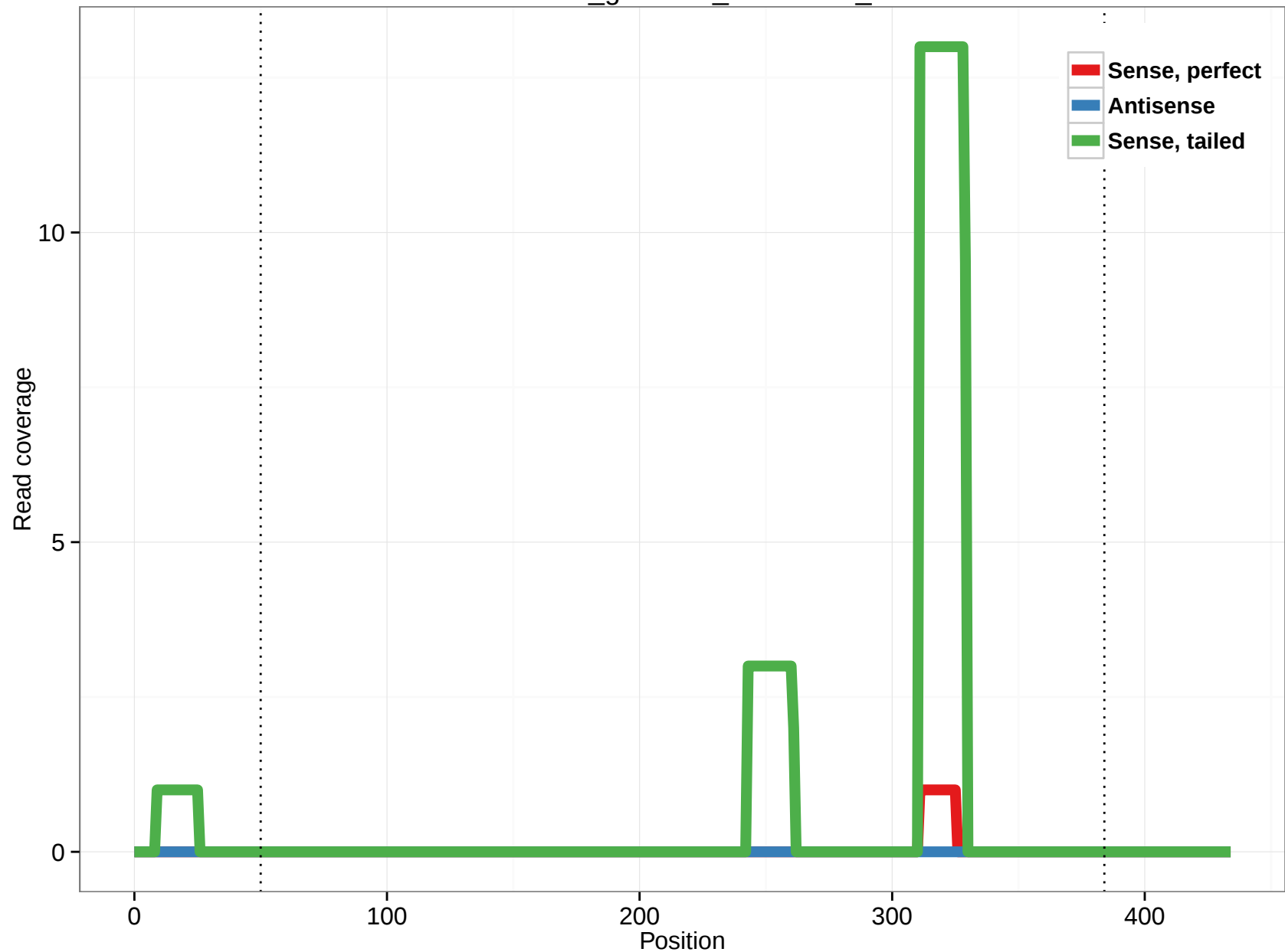
rheMac3_genscan_chr4.2485_5
