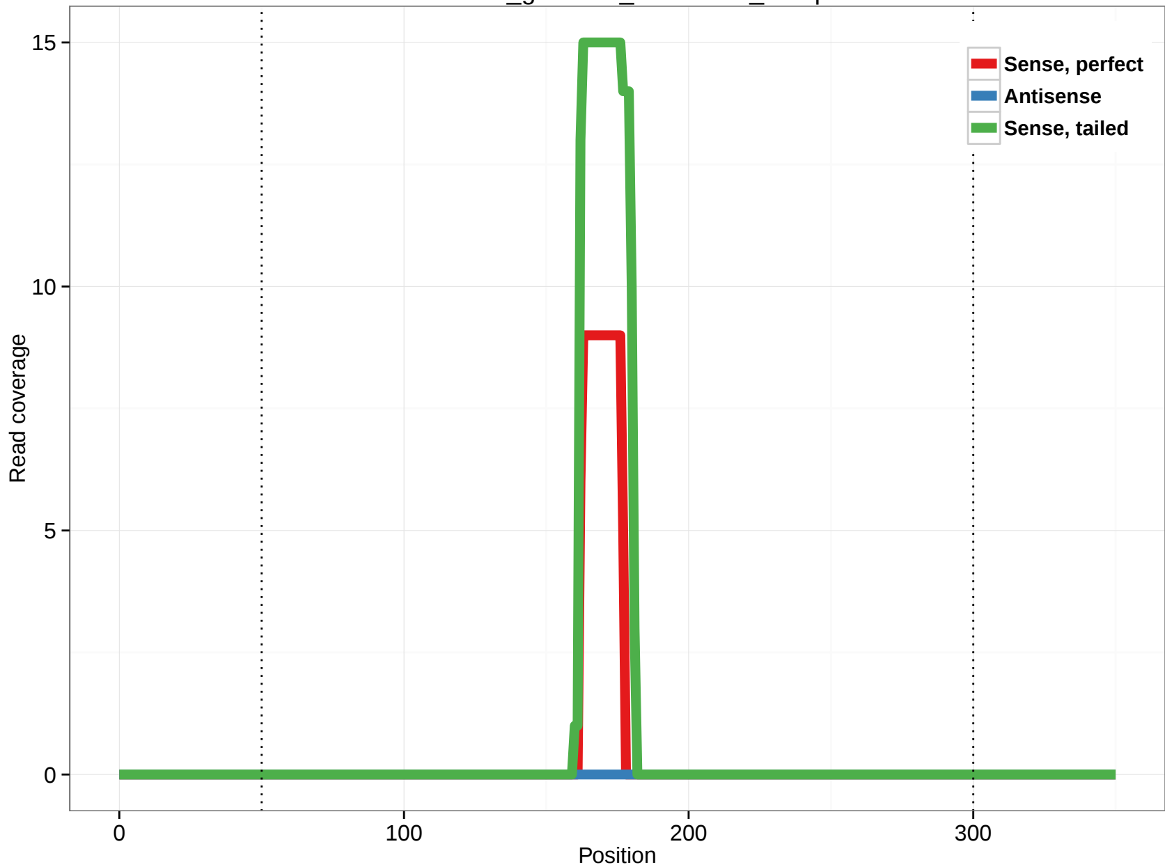
rheMac3_genscan_chr4.2321_22.5p
