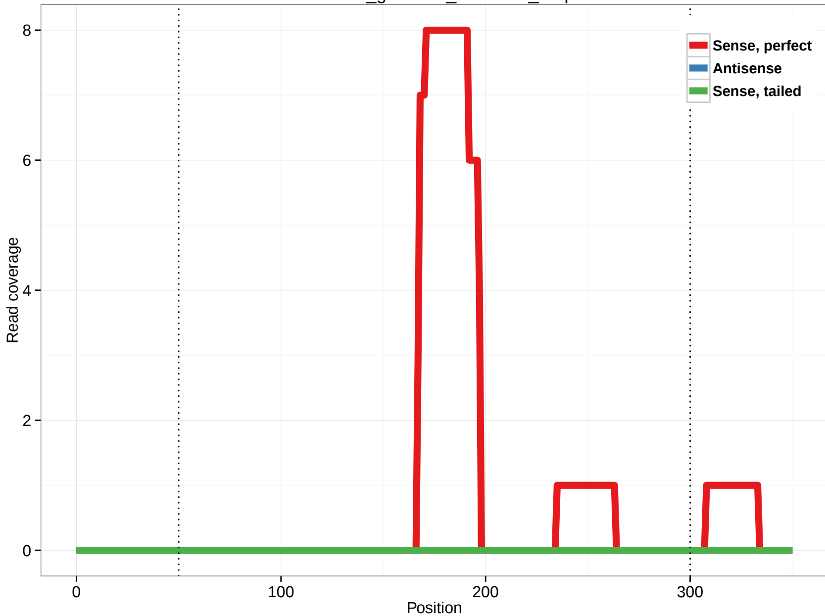
rheMac3_genscan_chr4.213_1.3p
