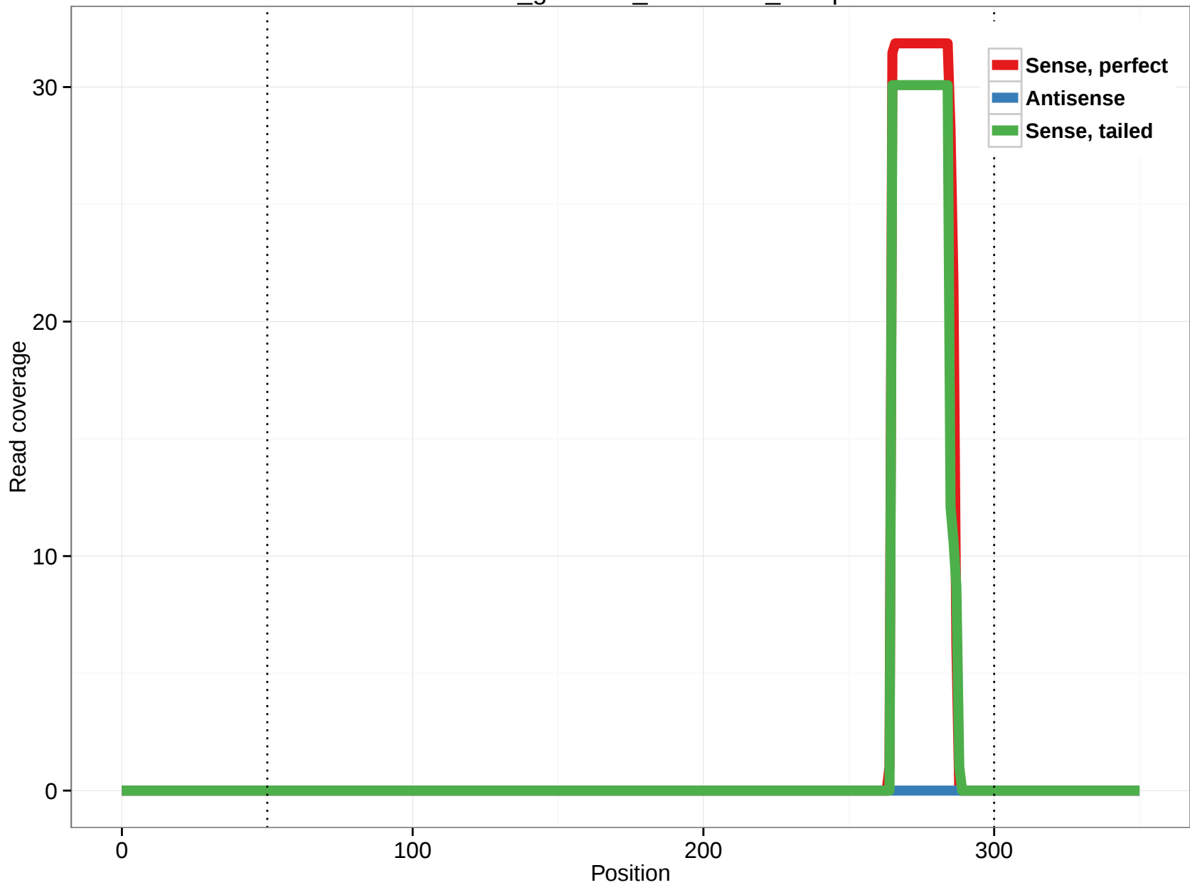
rheMac3_genscan_chr4.2060_12.3p
