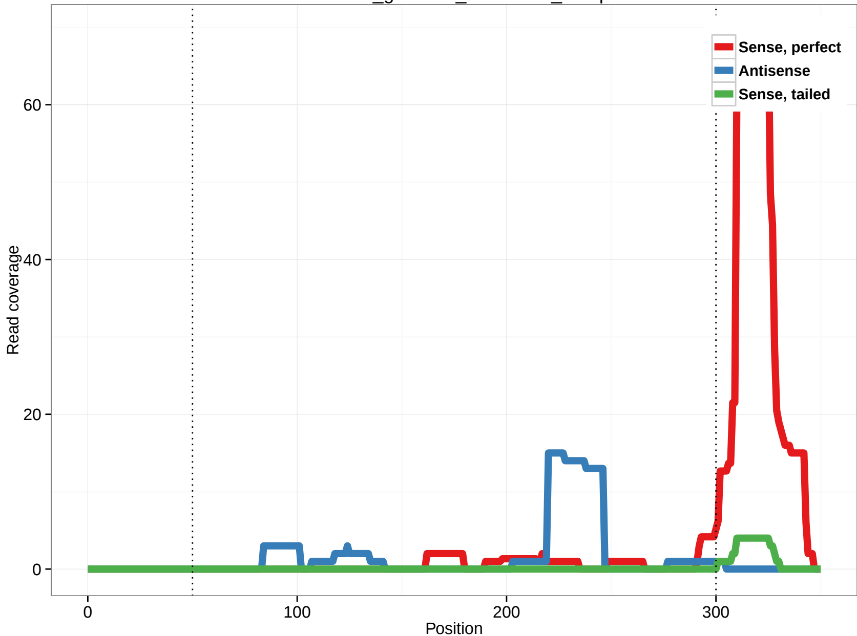
rheMac3_genscan_chr4.2020_15.3p
