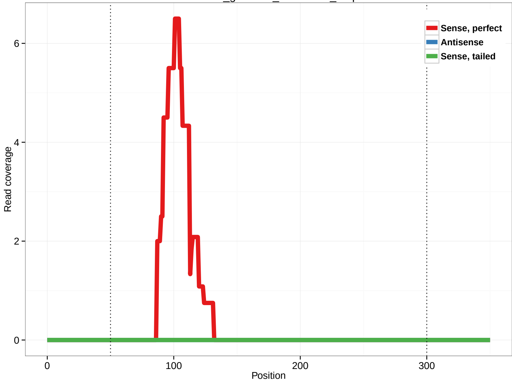
rheMac3_genscan_chr4.1857_1.5p
