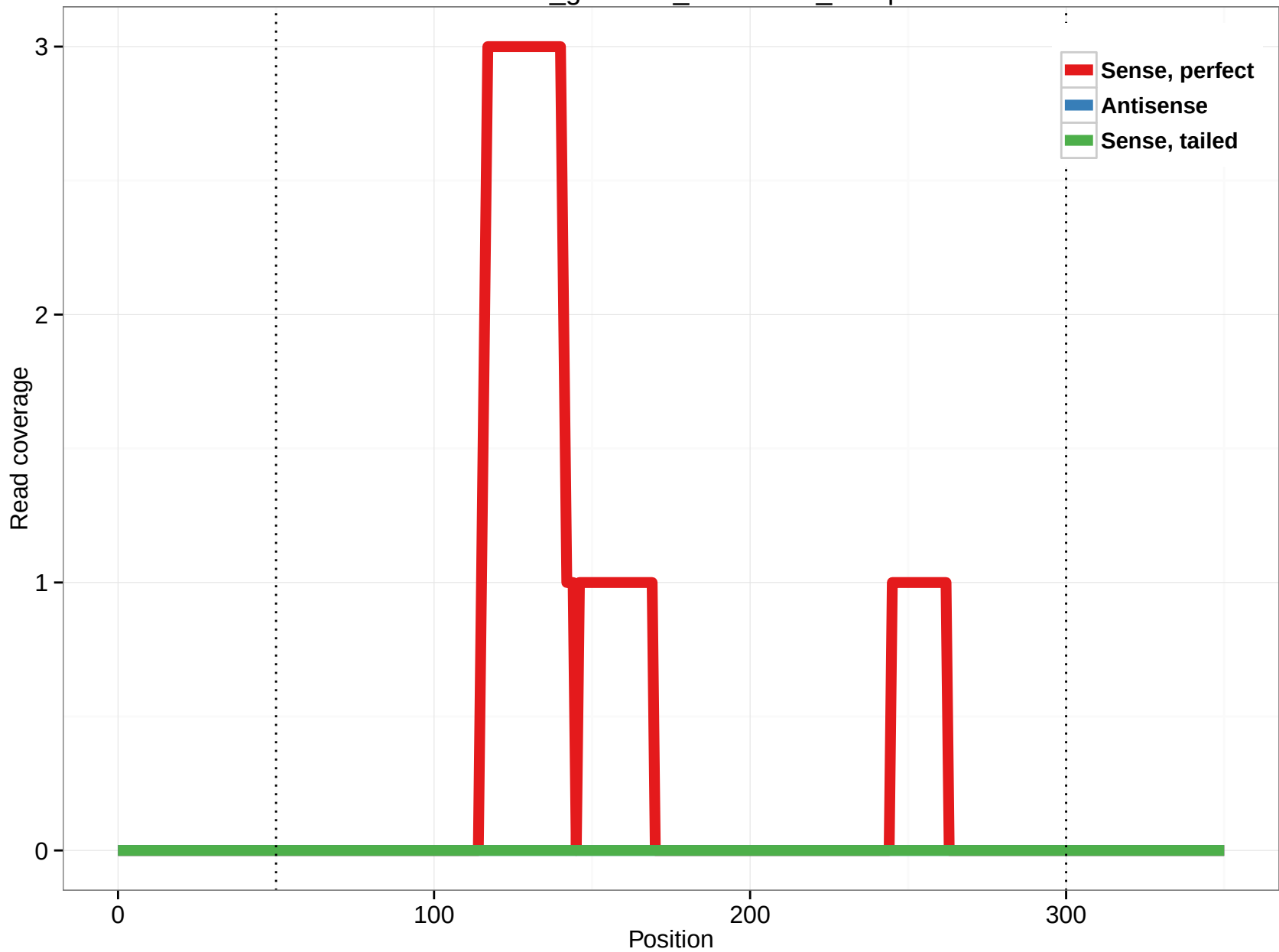
rheMac3_genscan_chr4.1810_16.5p
