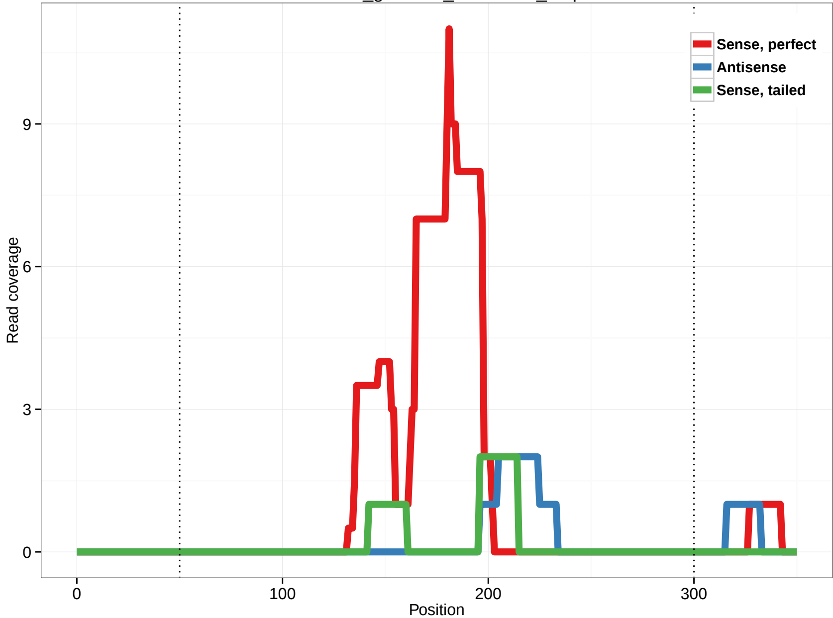
rheMac3_genscan_chr4.1717_2.3p
