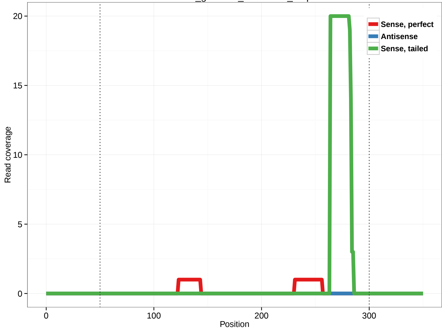
rheMac3_genscan_chr4.1626_0.5p
